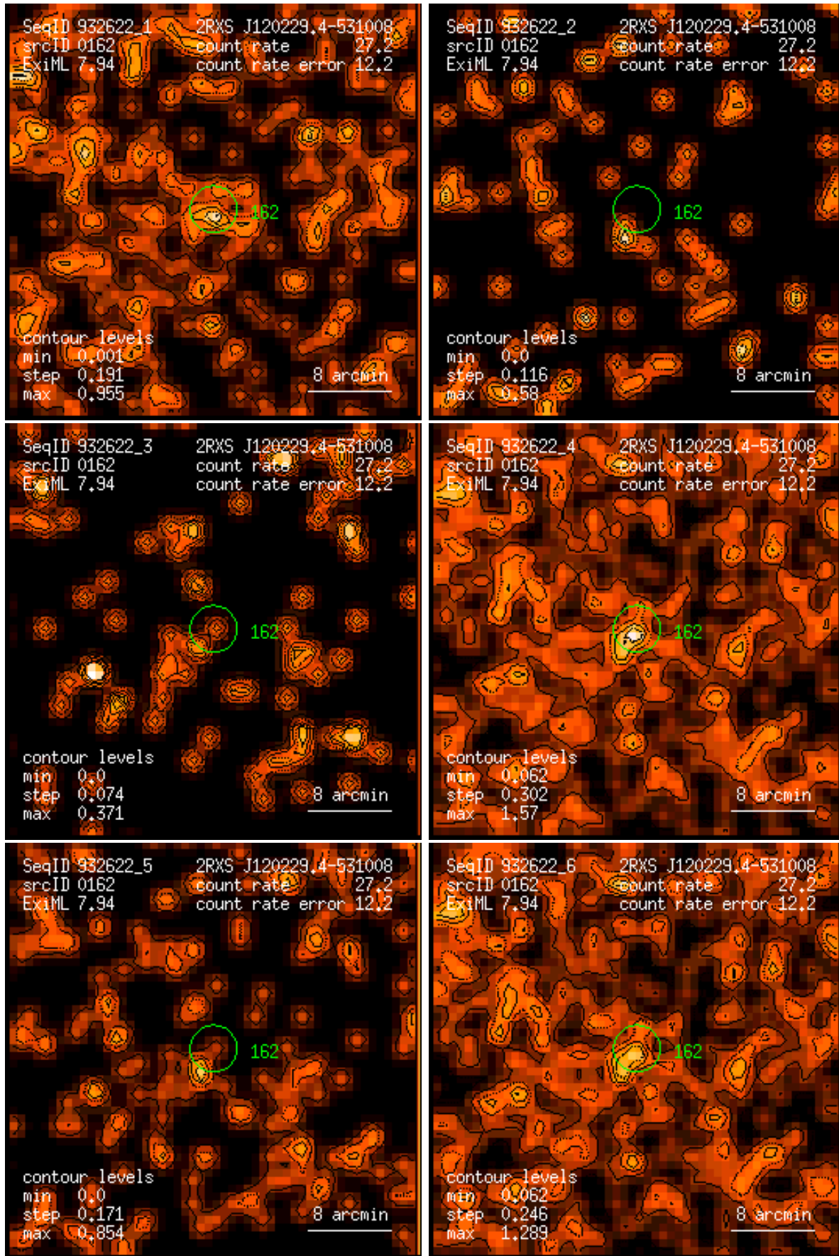
Figure 162: RASS 932622: detection 0162: band rate images, Gaussian filter: (1) PSPC channels 11 – 41, (2) 52 – 90, (3) 91 – 201, (4) 11 – 235, (5) 52 – 201, (6) 11 – 201. Broad band rates in counts/ks. Band rate contour levels in counts/ks/arcmin 2 .
