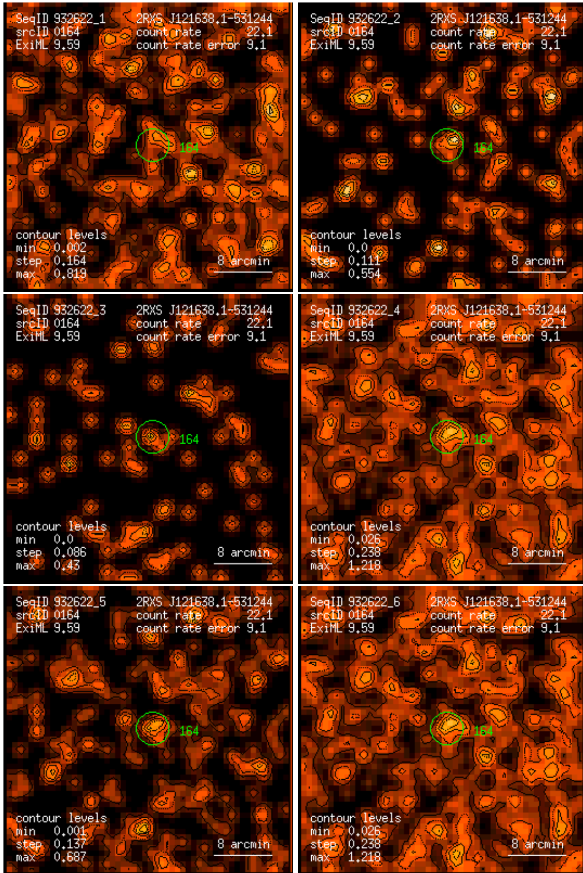
Figure 164: RASS 932622: detection 0164: band rate images, Gaussian filter: (1) PSPC channels 11 – 41, (2) 52 – 90, (3) 91 – 201, (4) 11 – 235, (5) 52 – 201, (6) 11 – 201. Broad band rates in counts/ks. Band rate contour levels in counts/ks/arcmin 2 .
