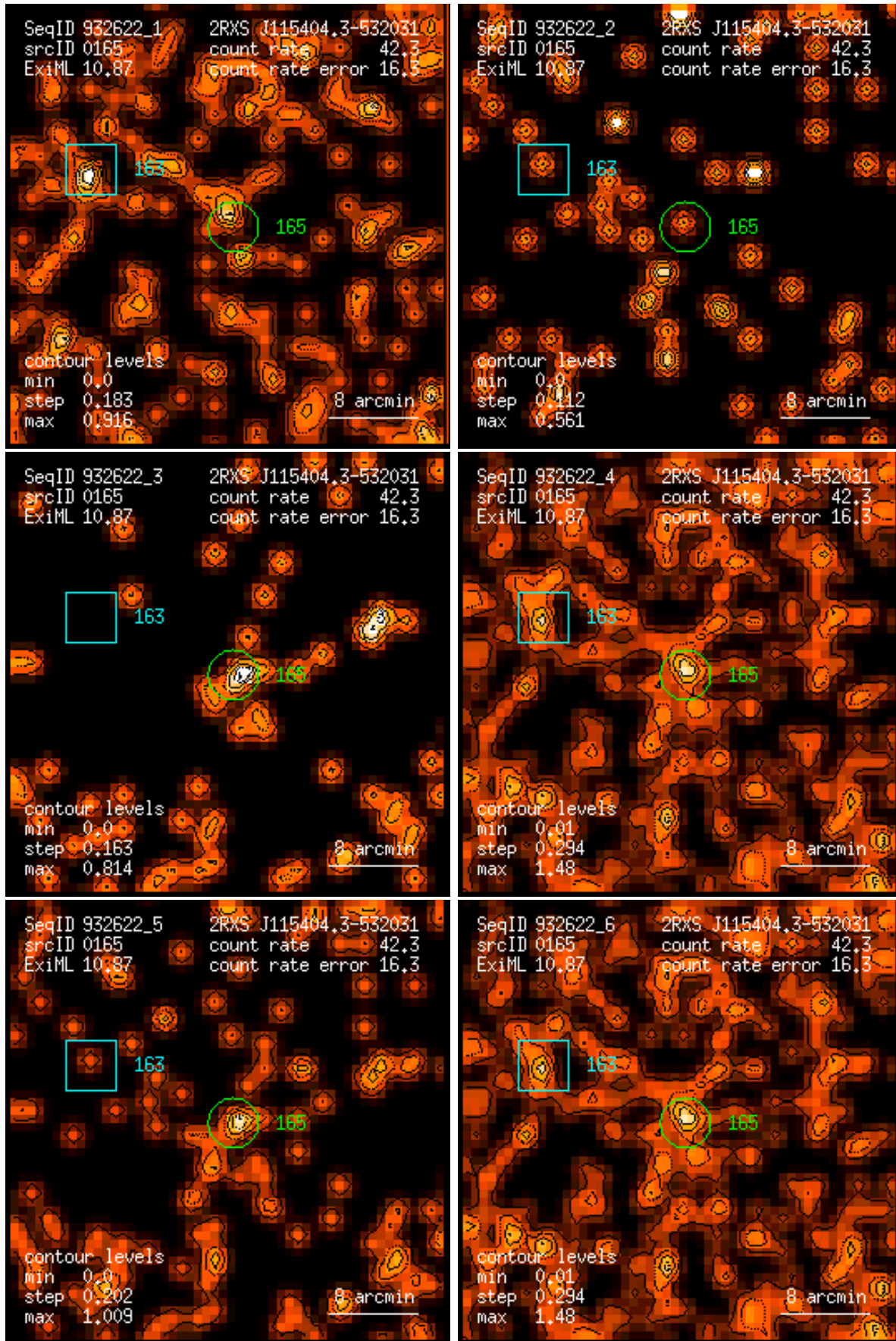
Figure 165: RASS 932622: detection 0165: band rate images, Gaussian filter: (1) PSPC channels 11 – 41, (2) 52 – 90, (3) 91 – 201, (4) 11 – 235, (5) 52 – 201, (6) 11 – 201. Broad band rates in counts/ks. Band rate contour levels in counts/ks/arcmin 2 .
