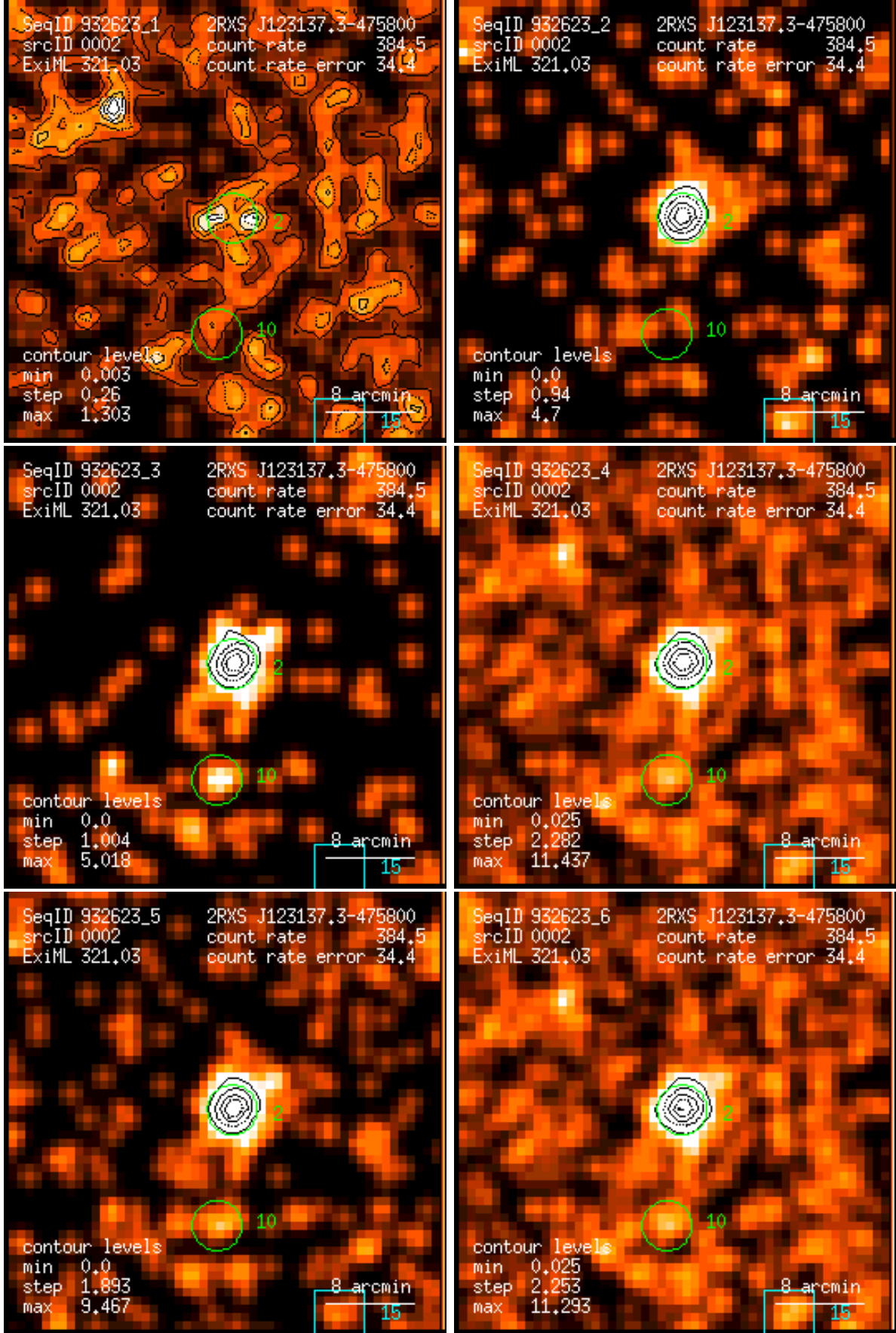
Figure 2: RASS 932623: detection 0002: band rate images, Gaussian filter: (1) PSPC channels 11 – 41, (2) 52 – 90, (3) 91 – 201, (4) 11 – 235, (5) 52 – 201, (6) 11 – 201. Broad band rates in counts/ks. Band rate contour levels in counts/ks/arcmin 2 .
