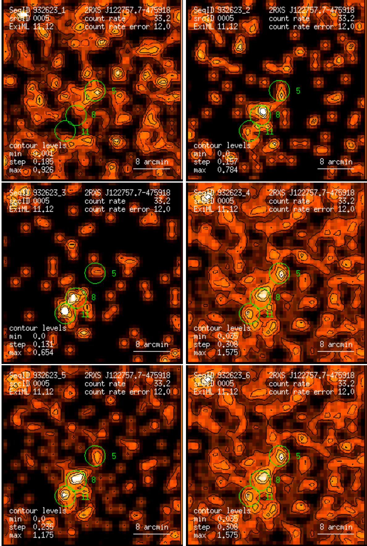
Figure 5: RASS 932623: detection 0005: band rate images, Gaussian filter: (1) PSPC channels 11 – 41, (2) 52 – 90, (3) 91 – 201, (4) 11 – 235, (5) 52 – 201, (6) 11 – 201. Broad band rates in counts/ks. Band rate contour levels in counts/ks/arcmin 2 .
