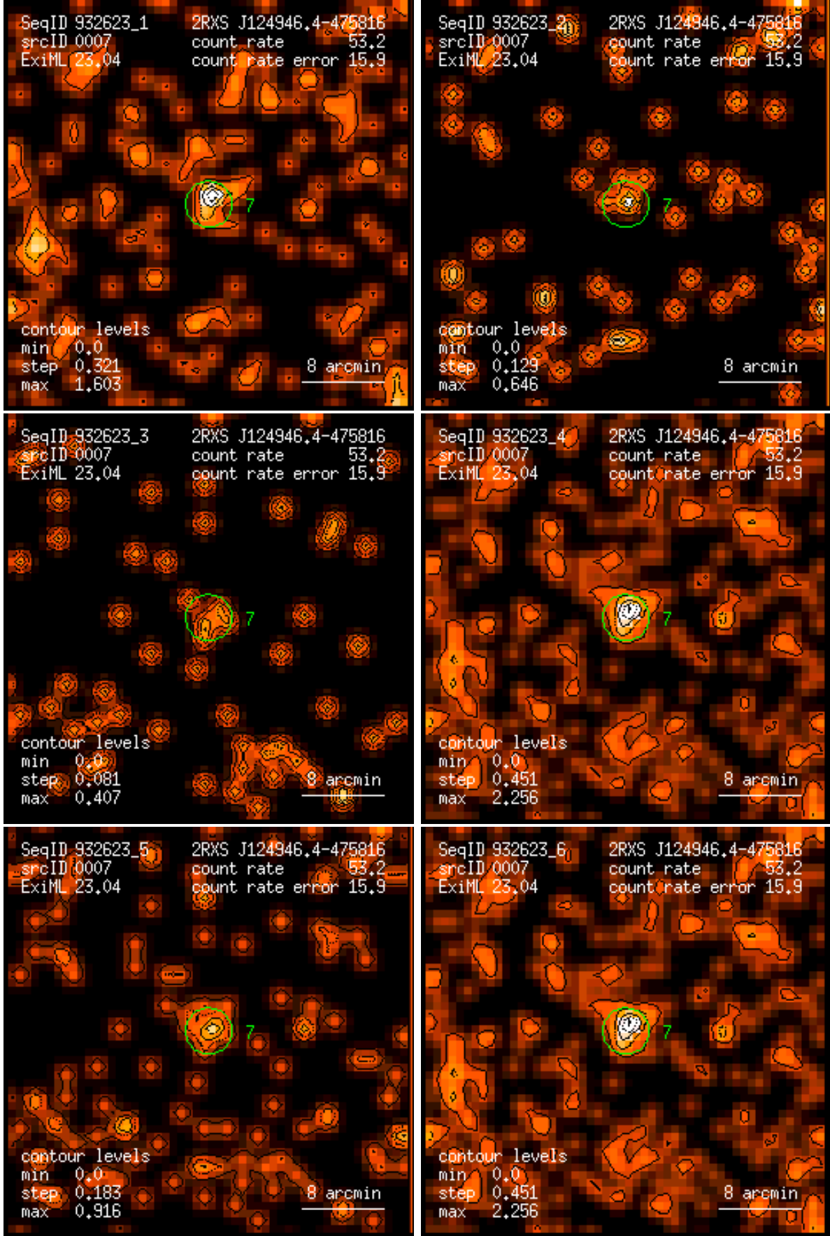
Figure 7: RASS 932623: detection 0007: band rate images, Gaussian filter: (1) PSPC channels 11 – 41, (2) 52 – 90, (3) 91 – 201, (4) 11 – 235, (5) 52 – 201, (6) 11 – 201. Broad band rates in counts/ks. Band rate contour levels in counts/ks/arcmin 2 .
