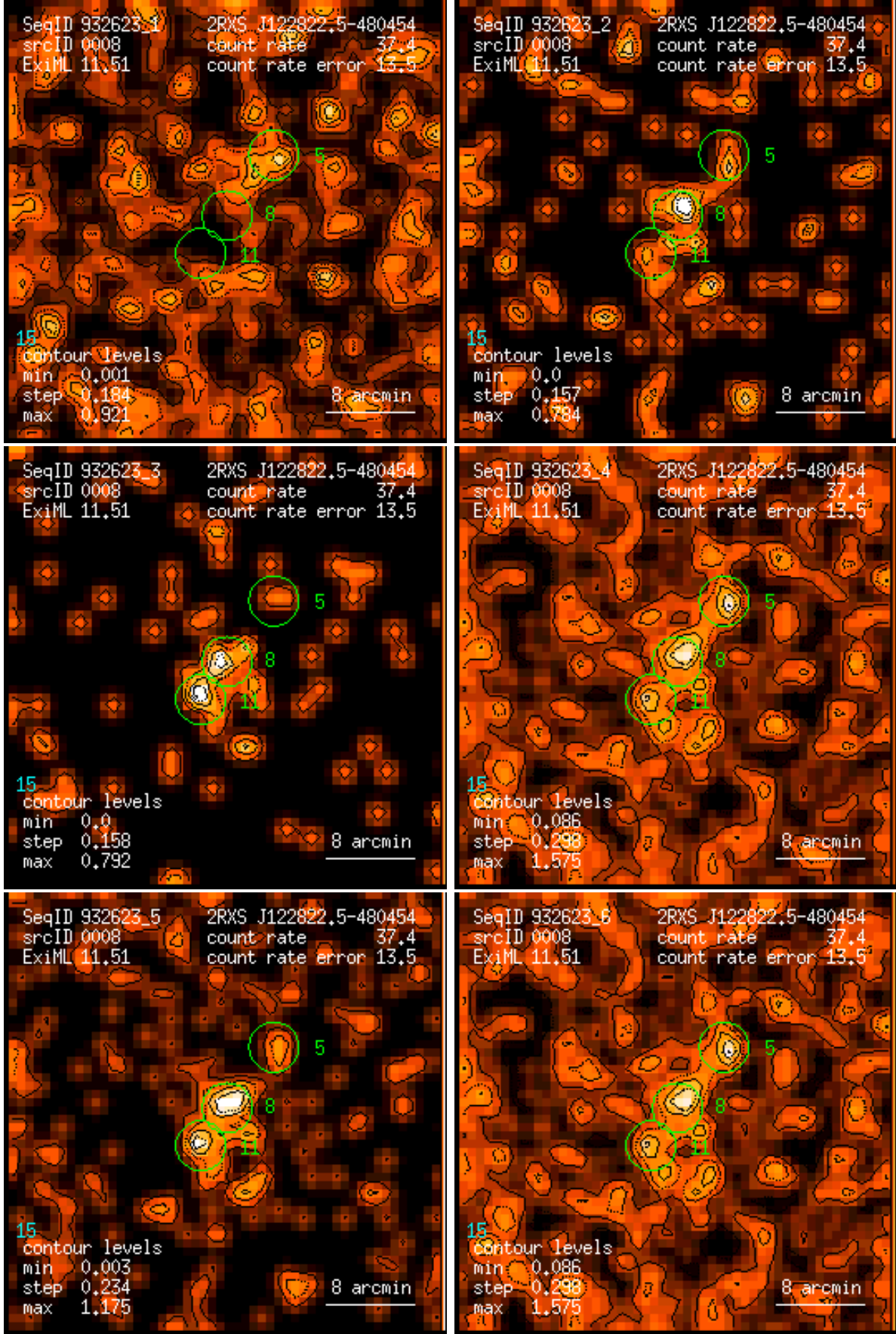
Figure 8: RASS 932623: detection 0008: band rate images, Gaussian filter: (1) PSPC channels 11 – 41, (2) 52 – 90, (3) 91 – 201, (4) 11 – 235, (5) 52 – 201, (6) 11 – 201. Broad band rates in counts/ks. Band rate contour levels in counts/ks/arcmin 2 .
