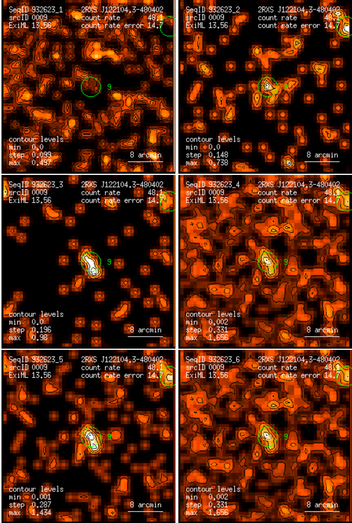
Figure 9: RASS 932623: detection 0009: band rate images, Gaussian filter: (1) PSPC channels 11 – 41, (2) 52 – 90, (3) 91 – 201, (4) 11 – 235, (5) 52 – 201, (6) 11 – 201. Broad band rates in counts/ks. Band rate contour levels in counts/ks/arcmin 2 .
