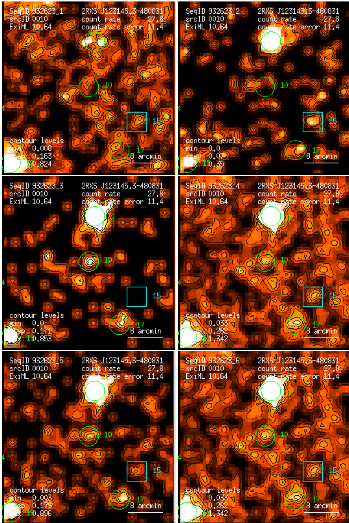
Figure 10: RASS 932623: detection 0010: band rate images, Gaussian filter: (1) PSPC channels 11 – 41, (2) 52 – 90, (3) 91 – 201, (4) 11 – 235, (5) 52 – 201, (6) 11 – 201. Broad band rates in counts/ks. Band rate contour levels in counts/ks/arcmin 2 .
