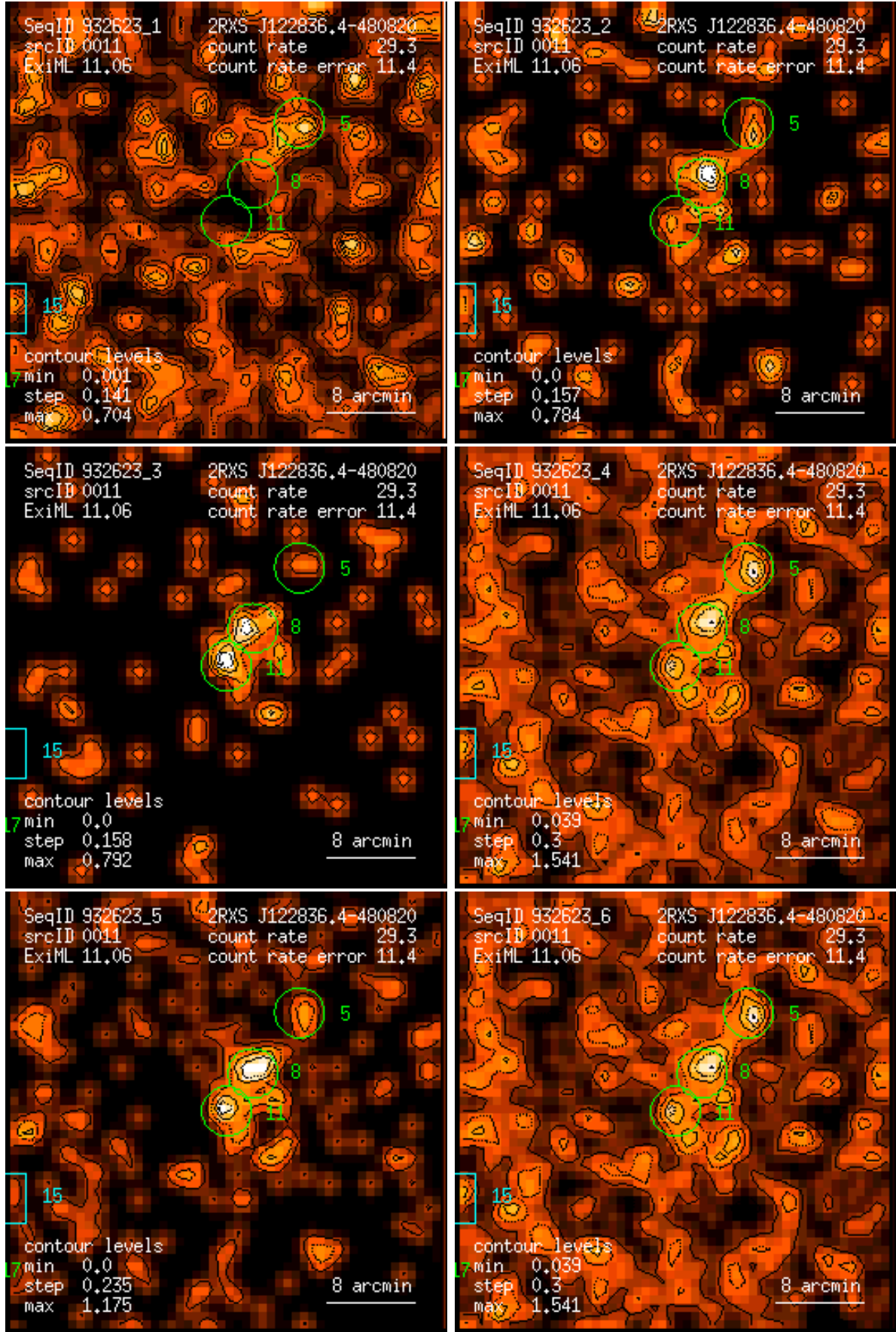
Figure 11: RASS 932623: detection 0011: band rate images, Gaussian filter: (1) PSPC channels 11 – 41, (2) 52 – 90, (3) 91 – 201, (4) 11 – 235, (5) 52 – 201, (6) 11 – 201. Broad band rates in counts/ks. Band rate contour levels in counts/ks/arcmin 2 .
