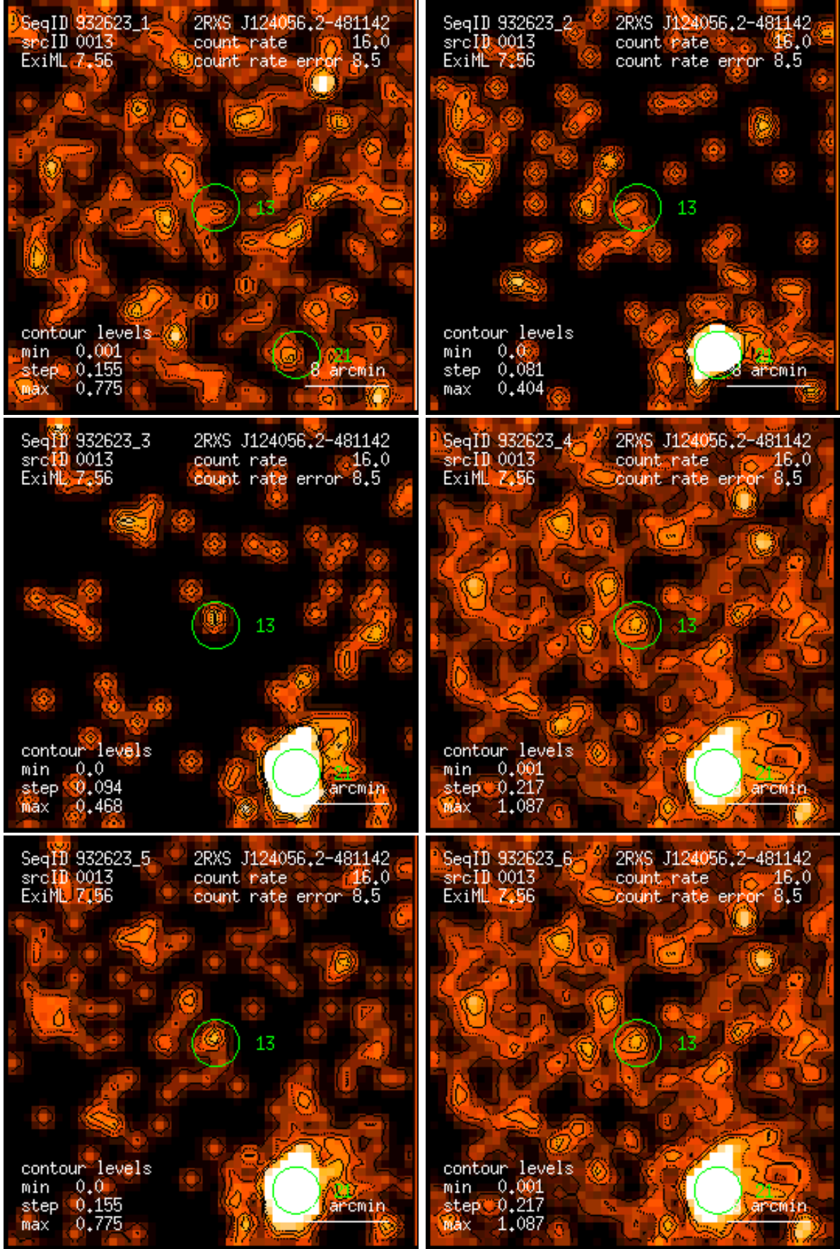
Figure 13: RASS 932623: detection 0013: band rate images, Gaussian filter: (1) PSPC channels 11 – 41, (2) 52 – 90, (3) 91 – 201, (4) 11 – 235, (5) 52 – 201, (6) 11 – 201. Broad band rates in counts/ks. Band rate contour levels in counts/ks/arcmin 2 .
