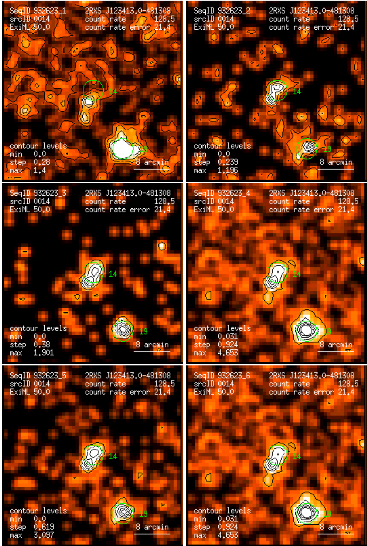
Figure 14: RASS 932623: detection 0014: band rate images, Gaussian filter: (1) PSPC channels 11 – 41, (2) 52 – 90, (3) 91 – 201, (4) 11 – 235, (5) 52 – 201, (6) 11 – 201. Broad band rates in counts/ks. Band rate contour levels in counts/ks/arcmin 2 .
