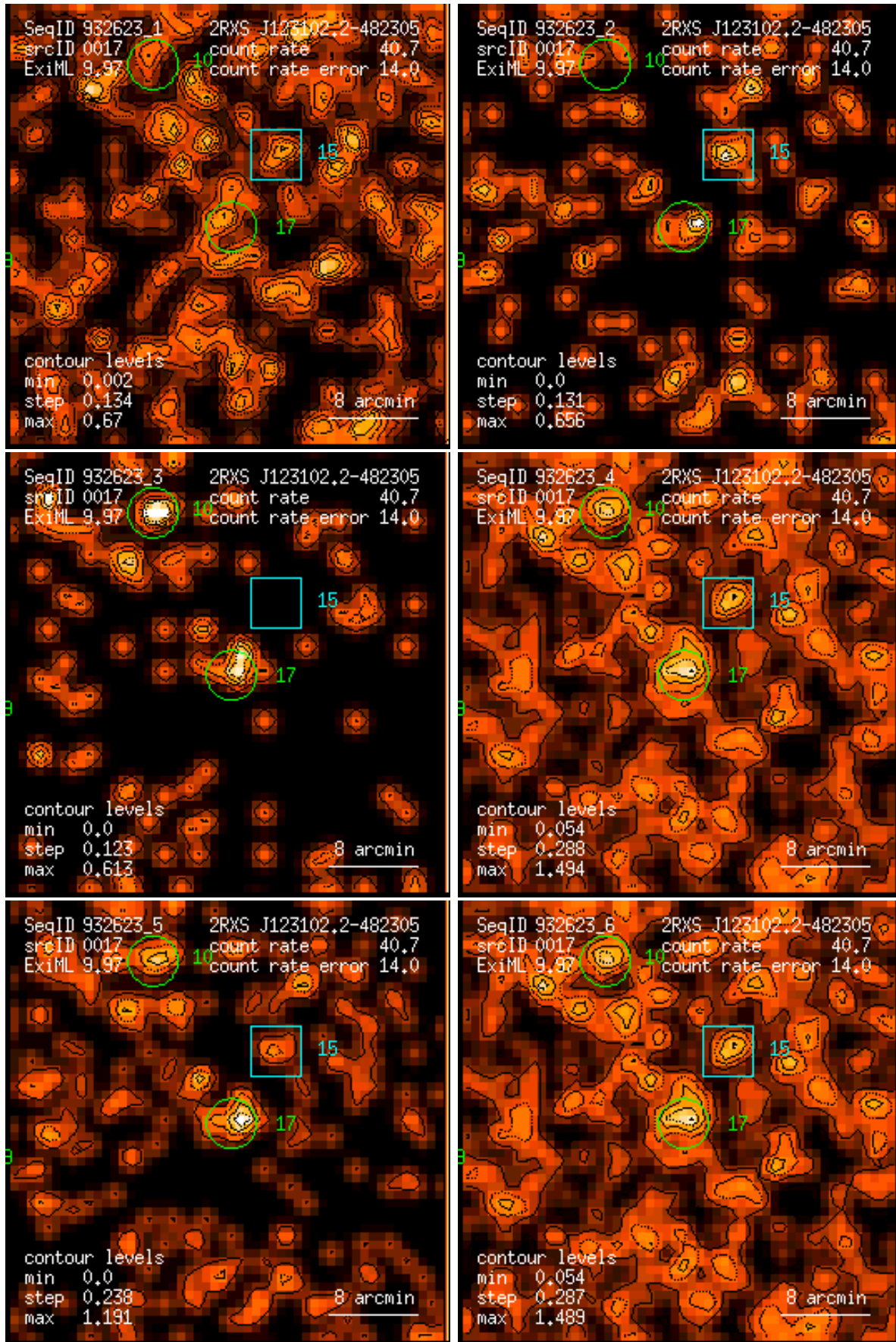
Figure 17: RASS 932623: detection 0017: band rate images, Gaussian filter: (1) PSPC channels 11 – 41, (2) 52 – 90, (3) 91 – 201, (4) 11 – 235, (5) 52 – 201, (6) 11 – 201. Broad band rates in counts/ks. Band rate contour levels in counts/ks/arcmin 2 .
