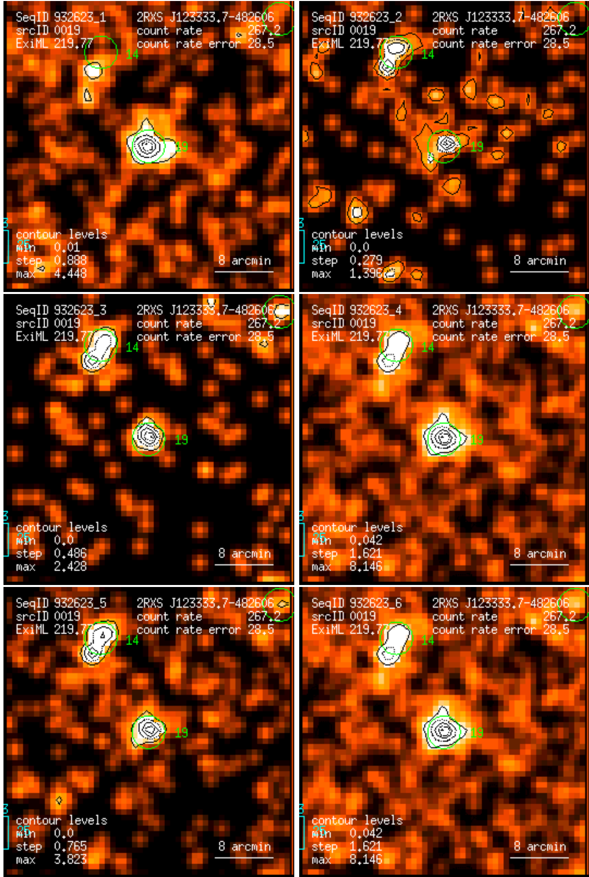
Figure 19: RASS 932623: detection 0019: band rate images, Gaussian filter: (1) PSPC channels 11 – 41, (2) 52 – 90, (3) 91 – 201, (4) 11 – 235, (5) 52 – 201, (6) 11 – 201. Broad band rates in counts/ks. Band rate contour levels in counts/ks/arcmin 2 .
