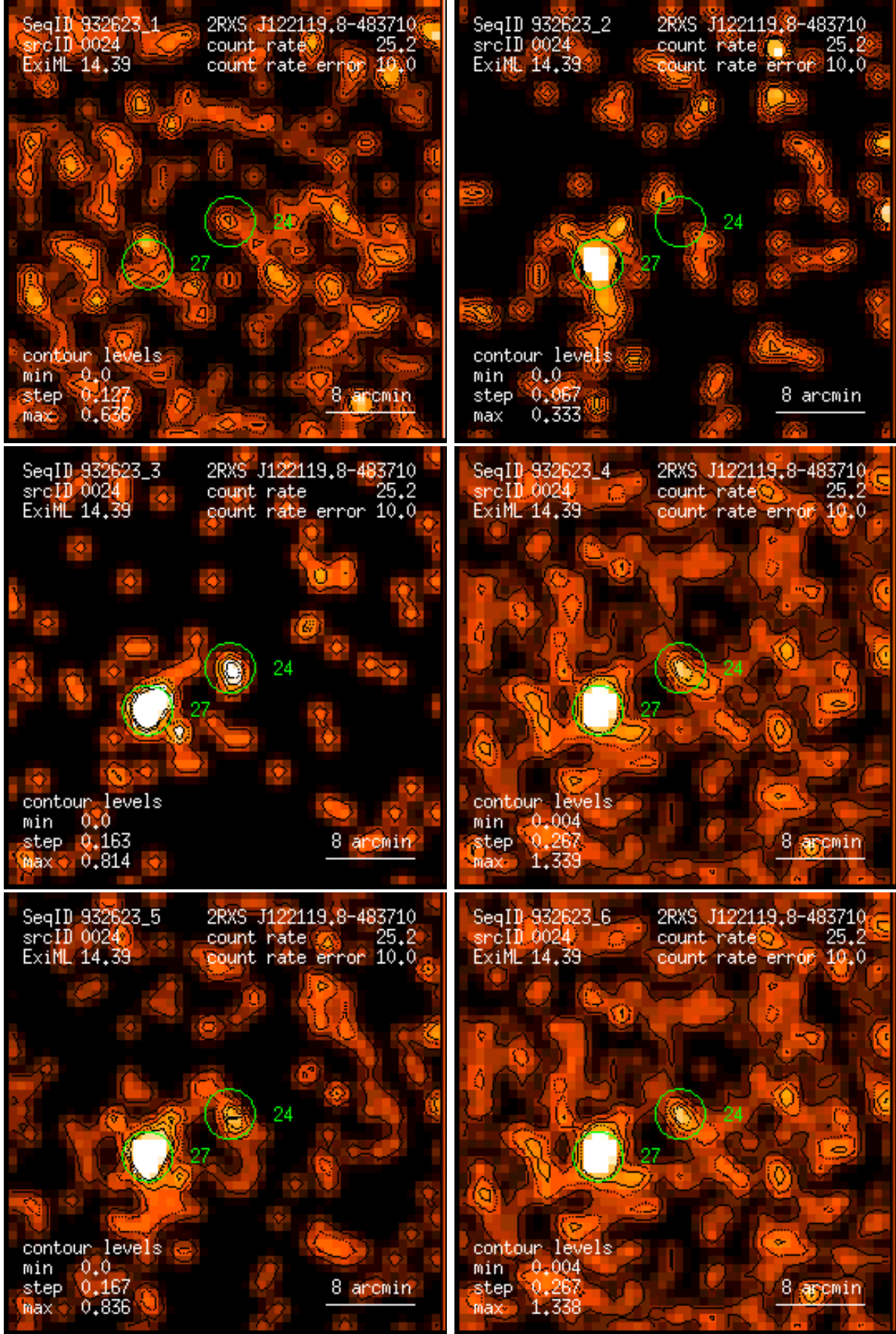
Figure 24: RASS 932623: detection 0024: band rate images, Gaussian filter: (1) PSPC channels 11 – 41, (2) 52 – 90, (3) 91 – 201, (4) 11 – 235, (5) 52 – 201, (6) 11 – 201. Broad band rates in counts/ks. Band rate contour levels in counts/ks/arcmin 2 .
