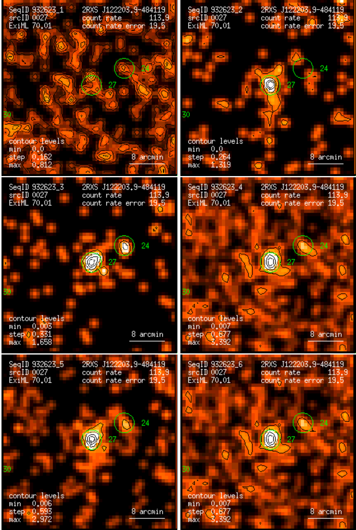
Figure 27: RASS 932623: detection 0027: band rate images, Gaussian filter: (1) PSPC channels 11 – 41, (2) 52 – 90, (3) 91 – 201, (4) 11 – 235, (5) 52 – 201, (6) 11 – 201. Broad band rates in counts/ks. Band rate contour levels in counts/ks/arcmin 2 .
