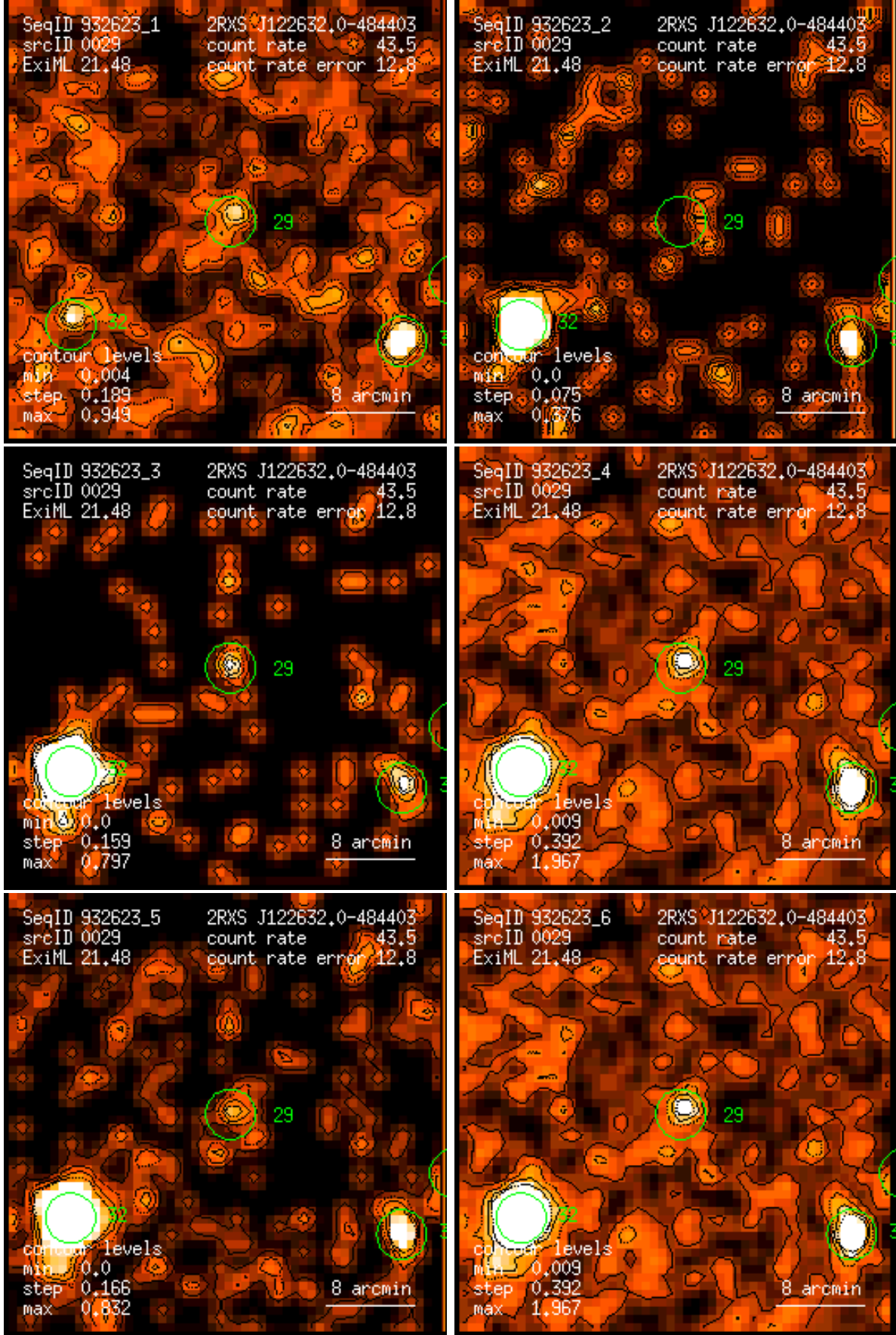
Figure 29: RASS 932623: detection 0029: band rate images, Gaussian filter: (1) PSPC channels 11 – 41, (2) 52 – 90, (3) 91 – 201, (4) 11 – 235, (5) 52 – 201, (6) 11 – 201. Broad band rates in counts/ks. Band rate contour levels in counts/ks/arcmin 2 .
