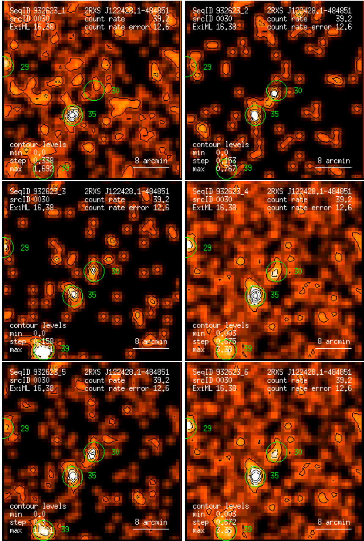
Figure 30: RASS 932623: detection 0030: band rate images, Gaussian filter: (1) PSPC channels 11 – 41, (2) 52 – 90, (3) 91 – 201, (4) 11 – 235, (5) 52 – 201, (6) 11 – 201. Broad band rates in counts/ks. Band rate contour levels in counts/ks/arcmin 2 .
