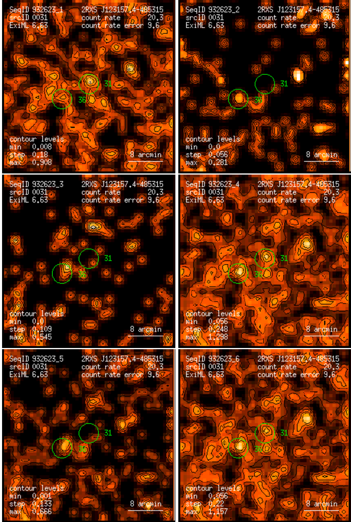
Figure 31: RASS 932623: detection 0031: band rate images, Gaussian filter: (1) PSPC channels 11 – 41, (2) 52 – 90, (3) 91 – 201, (4) 11 – 235, (5) 52 – 201, (6) 11 – 201. Broad band rates in counts/ks. Band rate contour levels in counts/ks/arcmin 2 .
