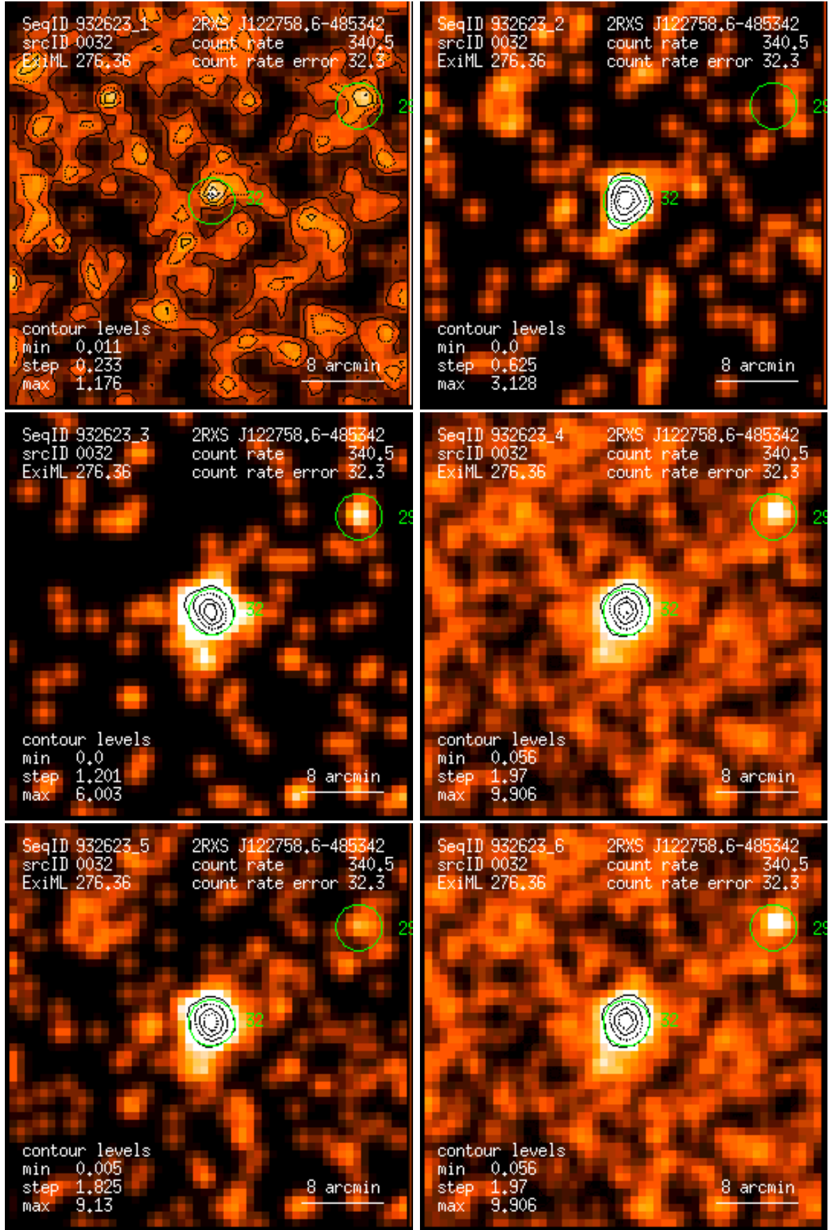
Figure 32: RASS 932623: detection 0032: band rate images, Gaussian filter: (1) PSPC channels 11 – 41, (2) 52 – 90, (3) 91 – 201, (4) 11 – 235, (5) 52 – 201, (6) 11 – 201. Broad band rates in counts/ks. Band rate contour levels in counts/ks/arcmin 2 .
