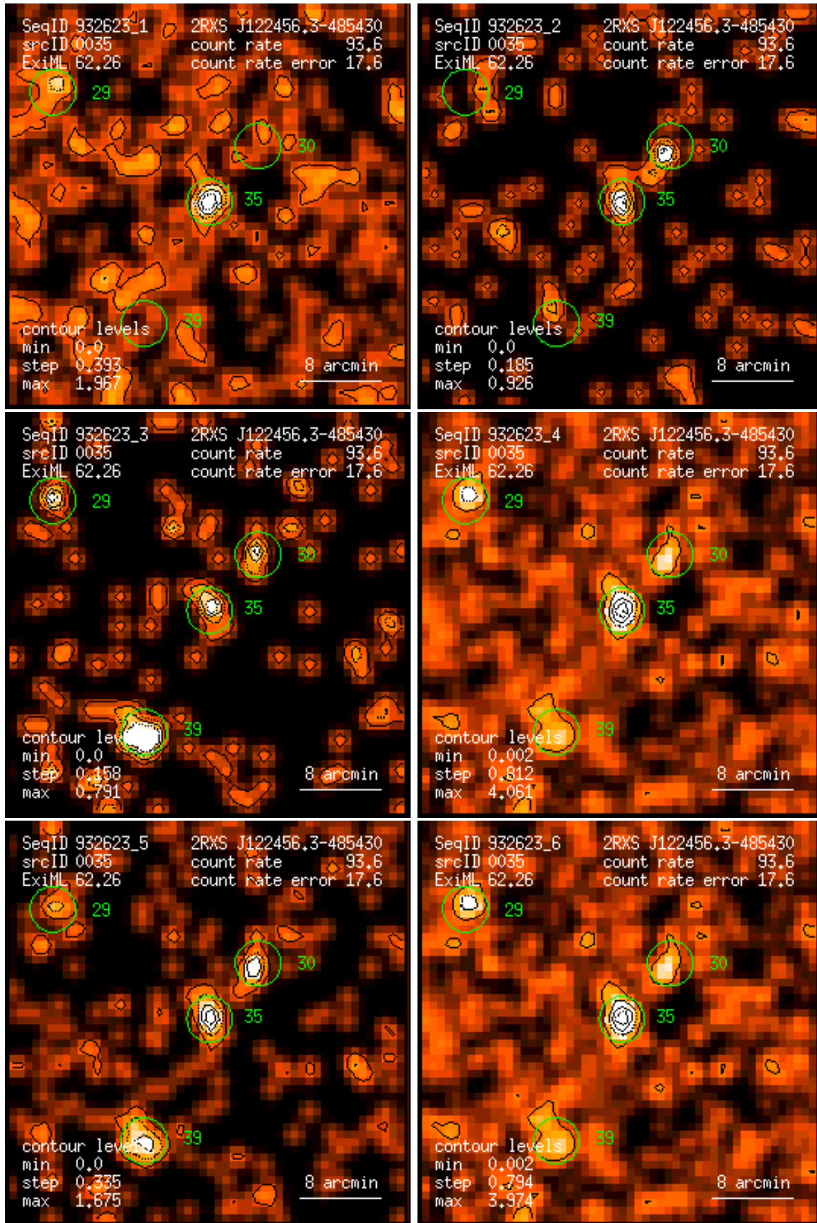
Figure 35: RASS 932623: detection 0035: band rate images, Gaussian filter: (1) PSPC channels 11 – 41, (2) 52 – 90, (3) 91 – 201, (4) 11 – 235, (5) 52 – 201, (6) 11 – 201. Broad band rates in counts/ks. Band rate contour levels in counts/ks/arcmin 2 .
