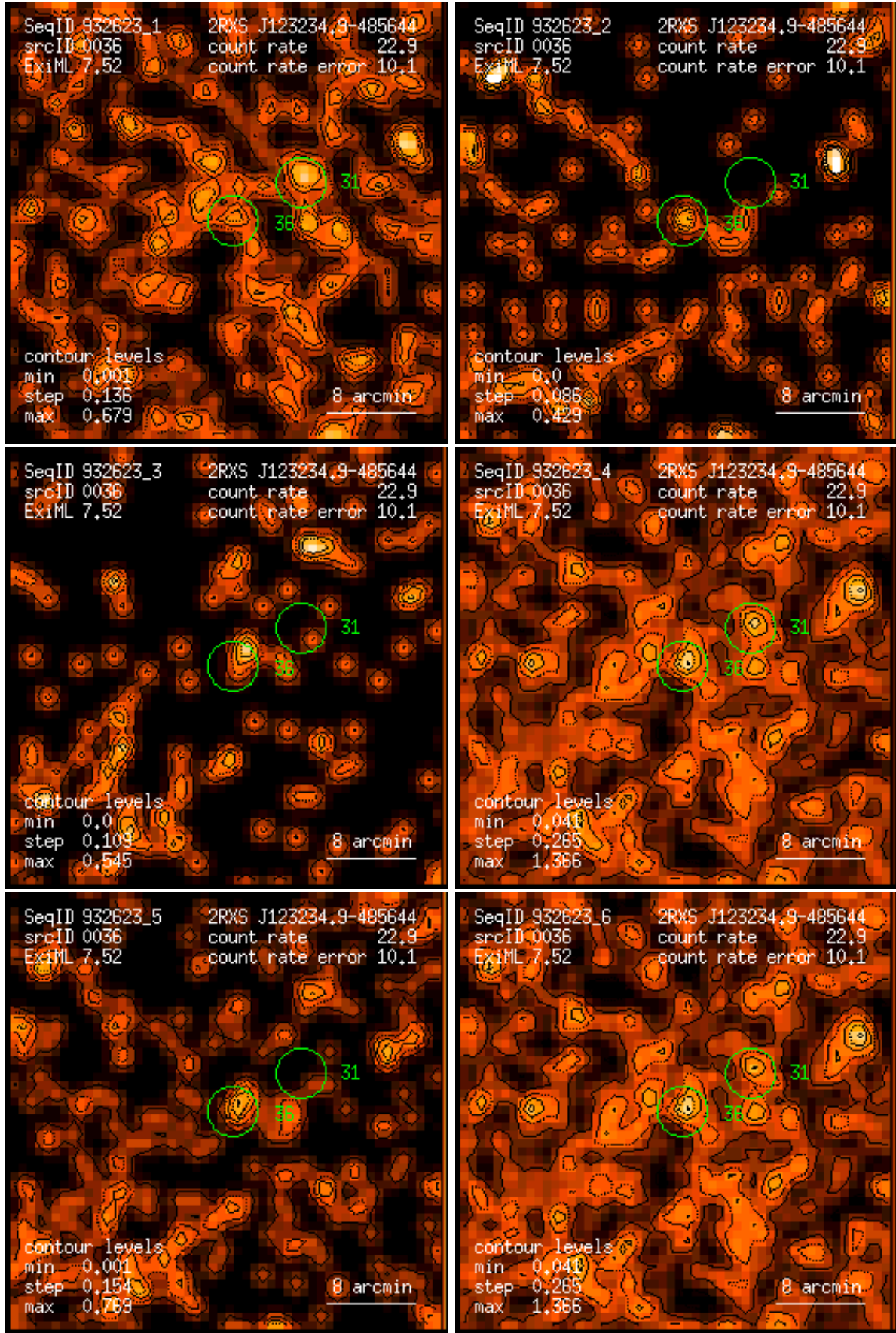
Figure 36: RASS 932623: detection 0036: band rate images, Gaussian filter: (1) PSPC channels 11 – 41, (2) 52 – 90, (3) 91 – 201, (4) 11 – 235, (5) 52 – 201, (6) 11 – 201. Broad band rates in counts/ks. Band rate contour levels in counts/ks/arcmin 2 .
