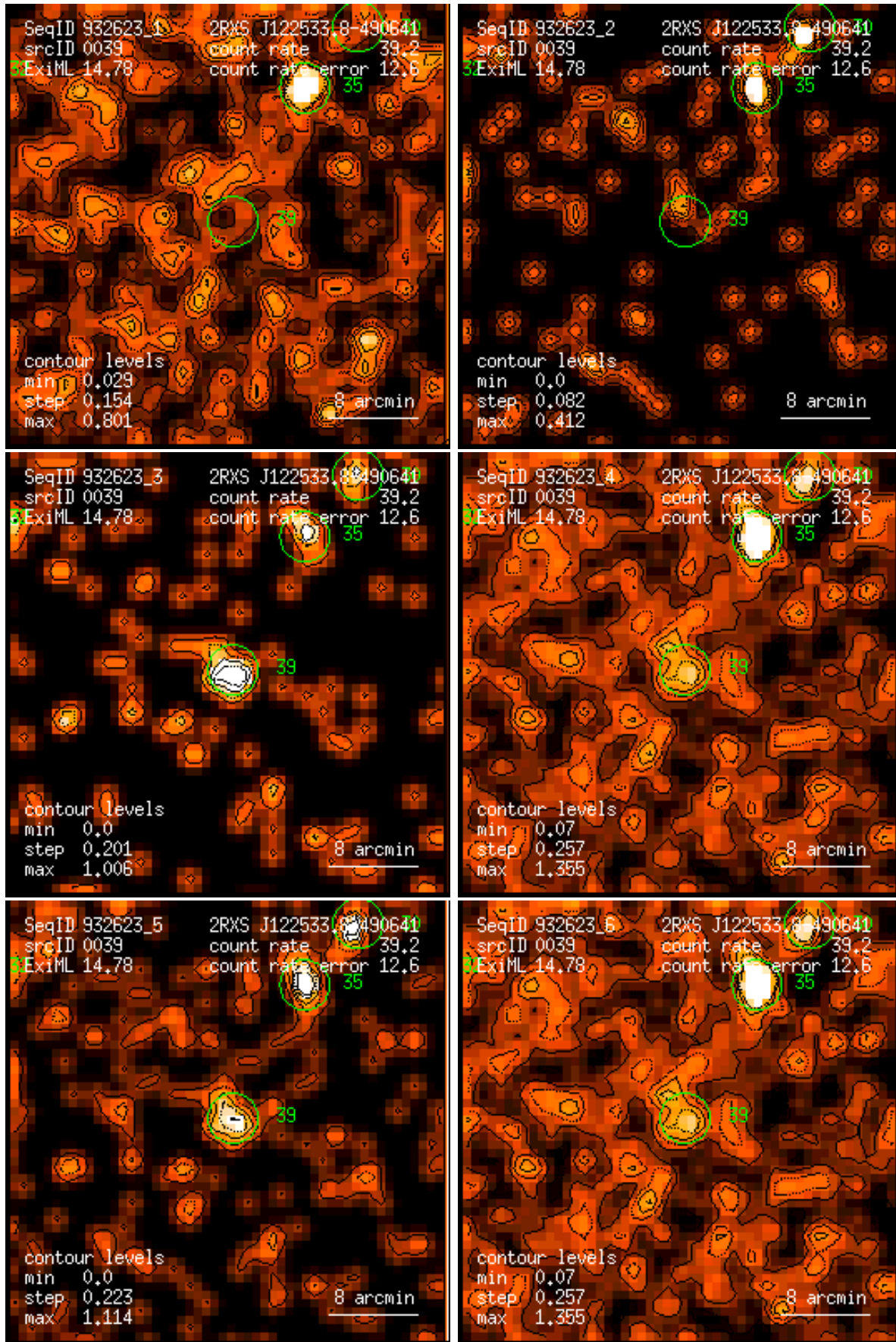
Figure 39: RASS 932623: detection 0039: band rate images, Gaussian filter: (1) PSPC channels 11 – 41, (2) 52 – 90, (3) 91 – 201, (4) 11 – 235, (5) 52 – 201, (6) 11 – 201. Broad band rates in counts/ks. Band rate contour levels in counts/ks/arcmin 2 .
