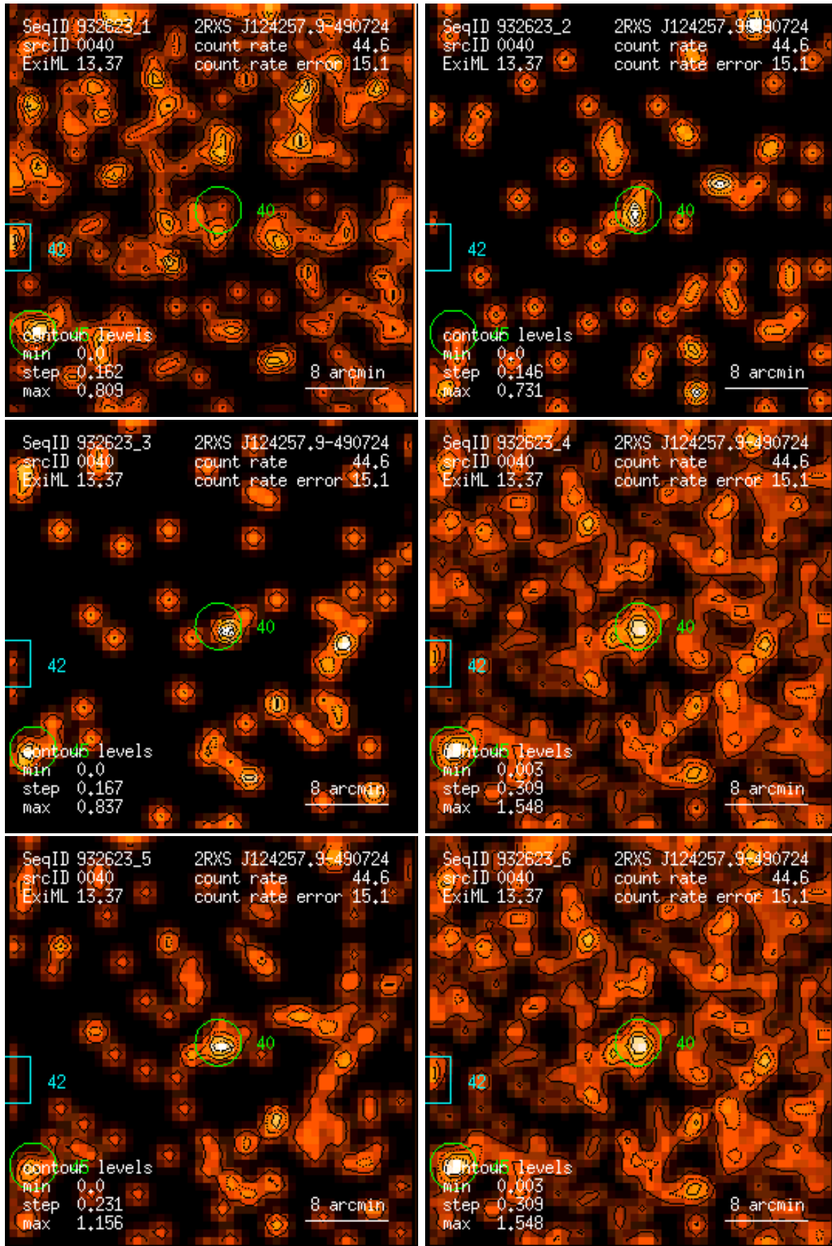
Figure 40: RASS 932623: detection 0040: band rate images, Gaussian filter: (1) PSPC channels 11 – 41, (2) 52 – 90, (3) 91 – 201, (4) 11 – 235, (5) 52 – 201, (6) 11 – 201. Broad band rates in counts/ks. Band rate contour levels in counts/ks/arcmin 2 .
