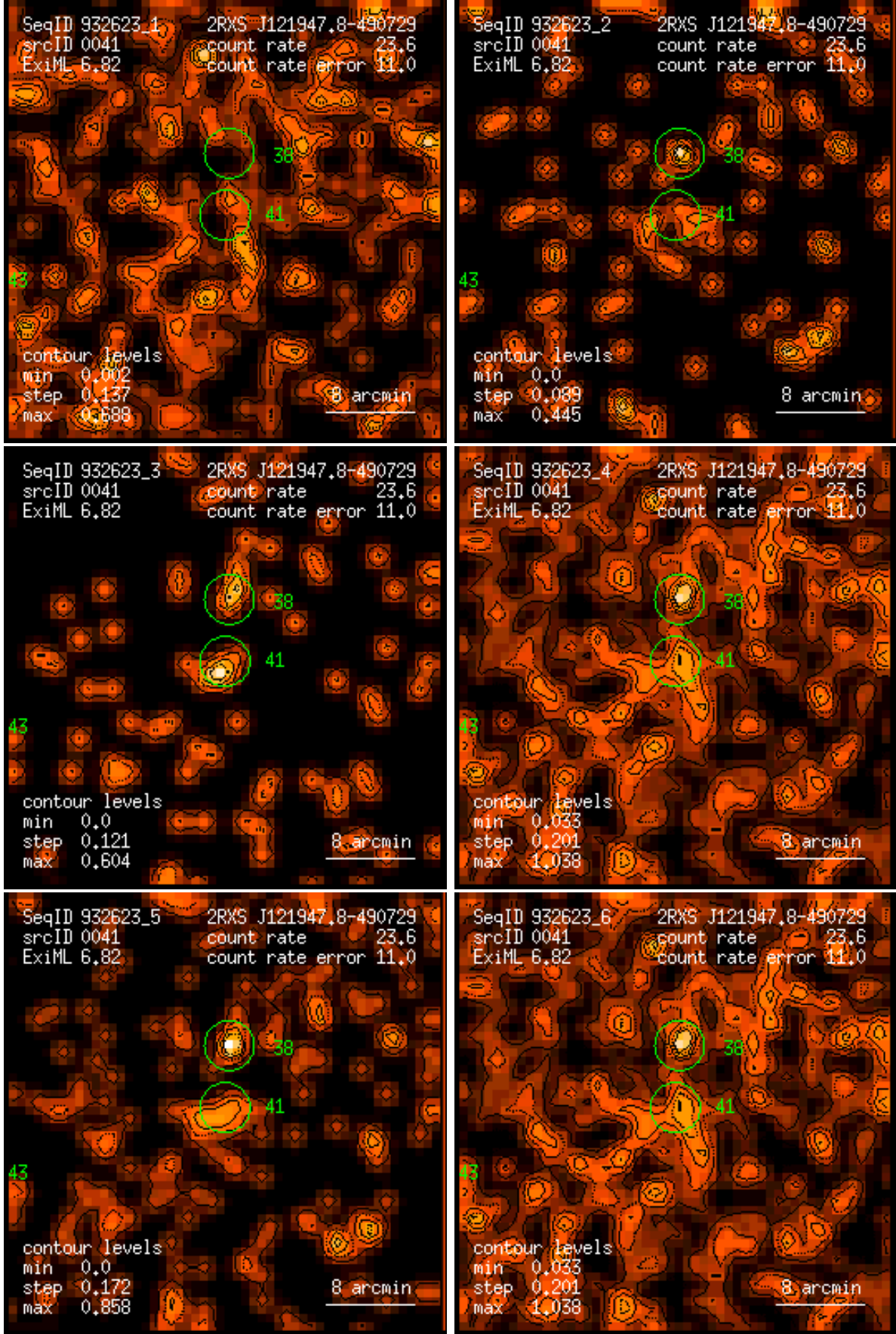
Figure 41: RASS 932623: detection 0041: band rate images, Gaussian filter: (1) PSPC channels 11 – 41, (2) 52 – 90, (3) 91 – 201, (4) 11 – 235, (5) 52 – 201, (6) 11 – 201. Broad band rates in counts/ks. Band rate contour levels in counts/ks/arcmin 2 .
