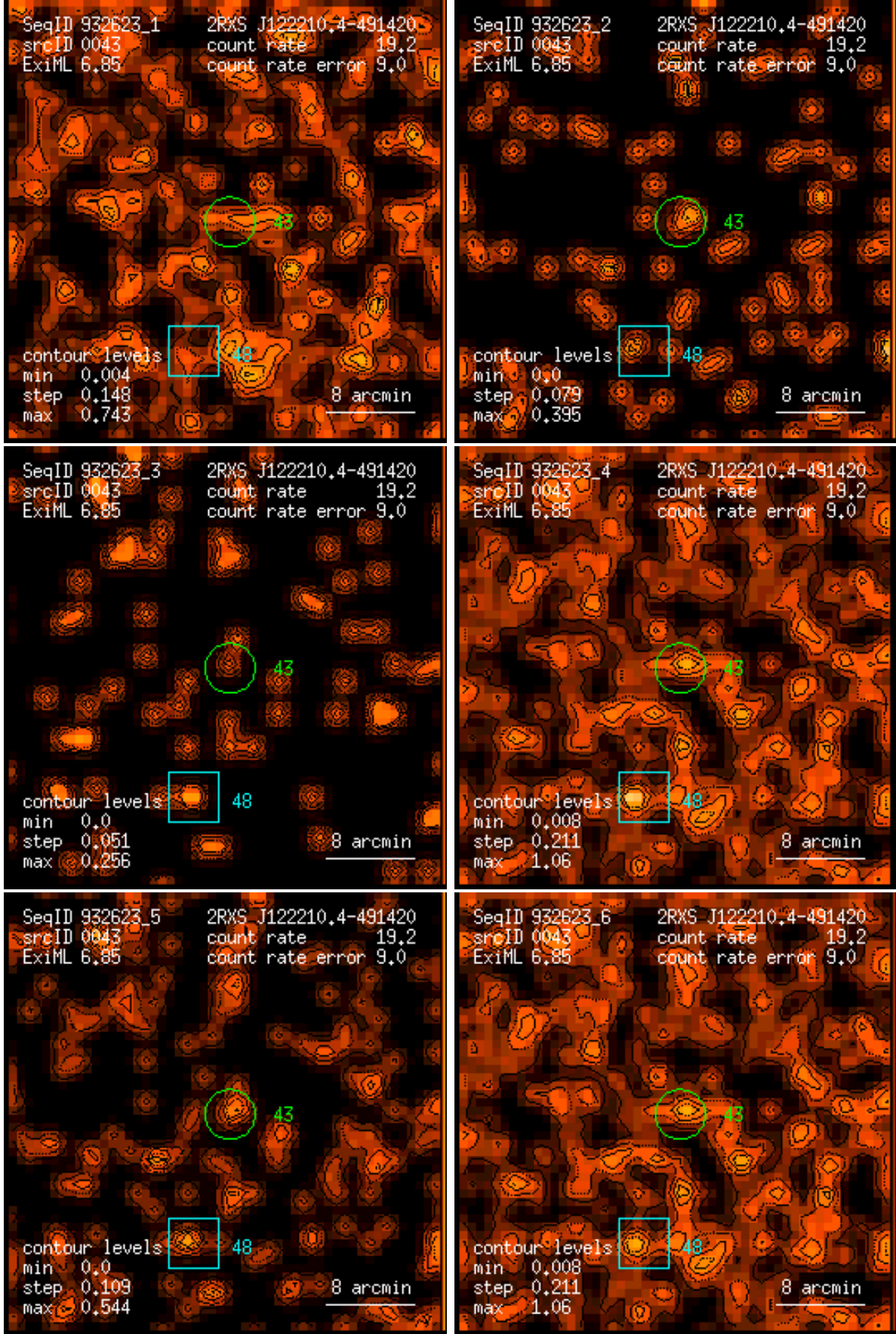
Figure 43: RASS 932623: detection 0043: band rate images, Gaussian filter: (1) PSPC channels 11 – 41, (2) 52 – 90, (3) 91 – 201, (4) 11 – 235, (5) 52 – 201, (6) 11 – 201. Broad band rates in counts/ks. Band rate contour levels in counts/ks/arcmin 2 .
