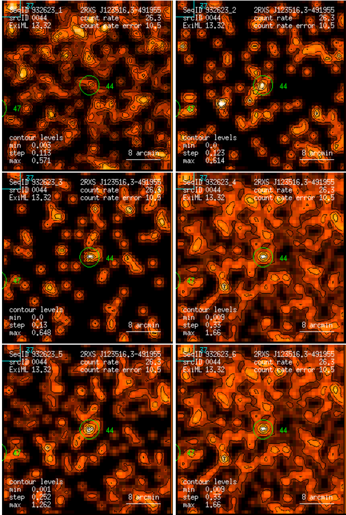
Figure 44: RASS 932623: detection 0044: band rate images, Gaussian filter: (1) PSPC channels 11 – 41, (2) 52 – 90, (3) 91 – 201, (4) 11 – 235, (5) 52 – 201, (6) 11 – 201. Broad band rates in counts/ks. Band rate contour levels in counts/ks/arcmin 2 .
