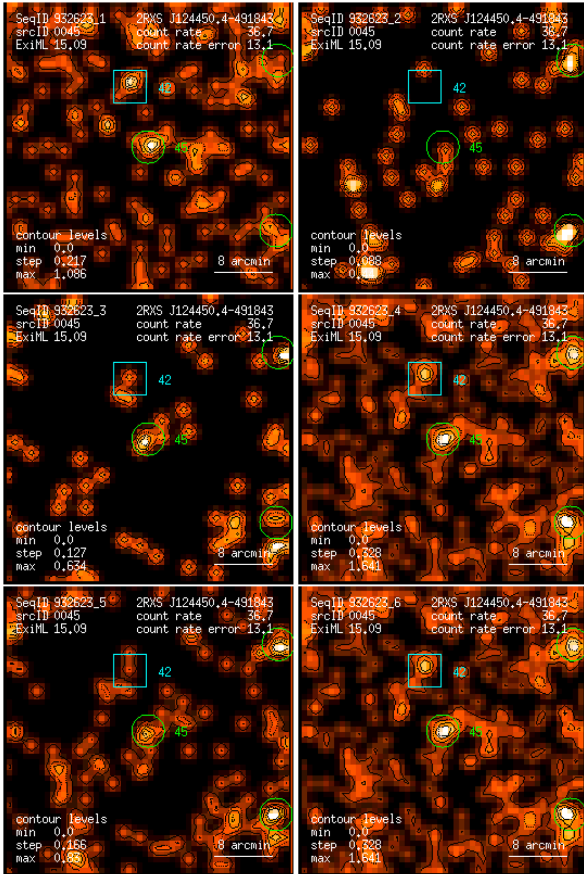
Figure 45: RASS 932623: detection 0045: band rate images, Gaussian filter: (1) PSPC channels 11 – 41, (2) 52 – 90, (3) 91 – 201, (4) 11 – 235, (5) 52 – 201, (6) 11 – 201. Broad band rates in counts/ks. Band rate contour levels in counts/ks/arcmin 2 .
