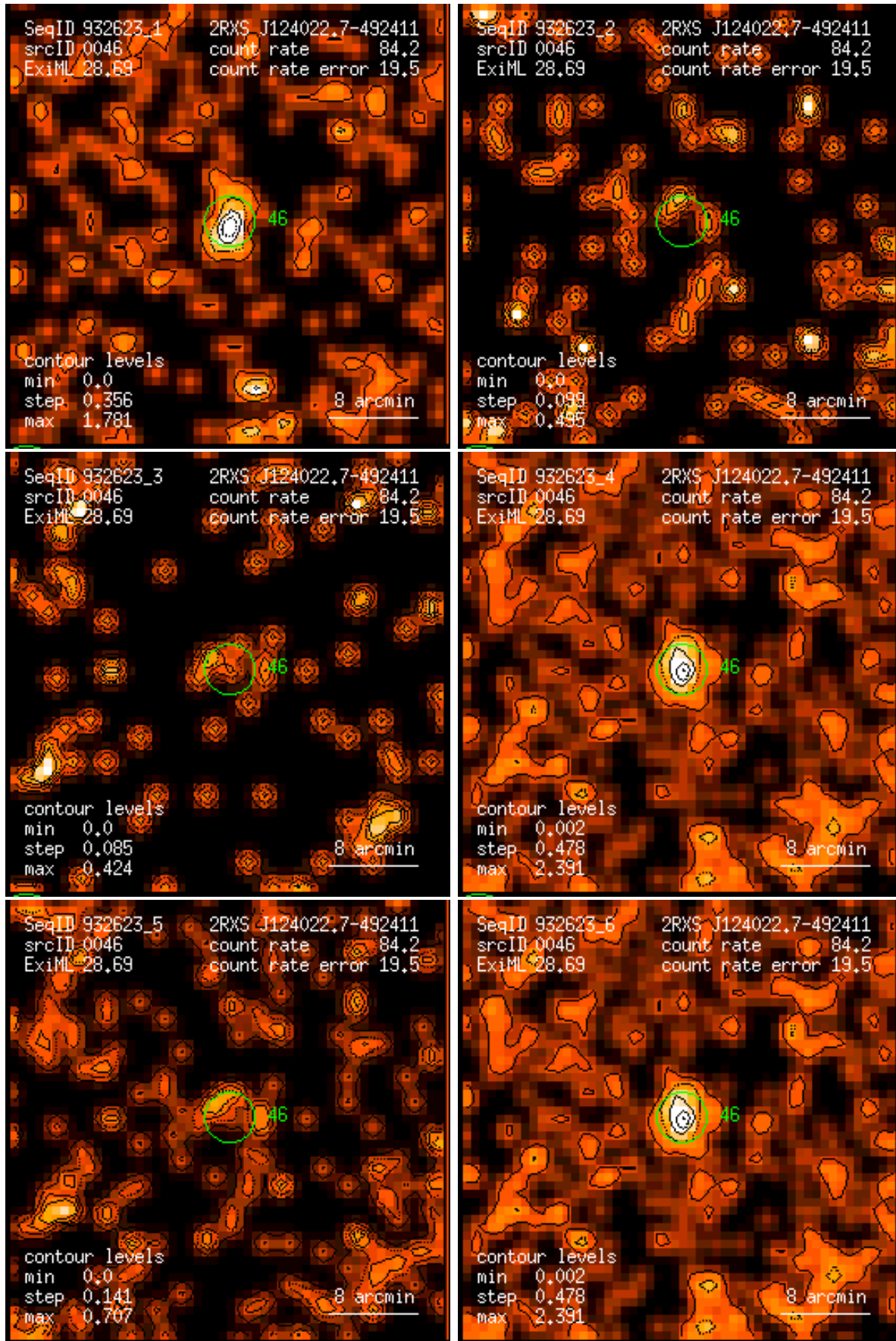
Figure 46: RASS 932623: detection 0046: band rate images, Gaussian filter: (1) PSPC channels 11 – 41, (2) 52 – 90, (3) 91 – 201, (4) 11 – 235, (5) 52 – 201, (6) 11 – 201. Broad band rates in counts/ks. Band rate contour levels in counts/ks/arcmin 2 .
