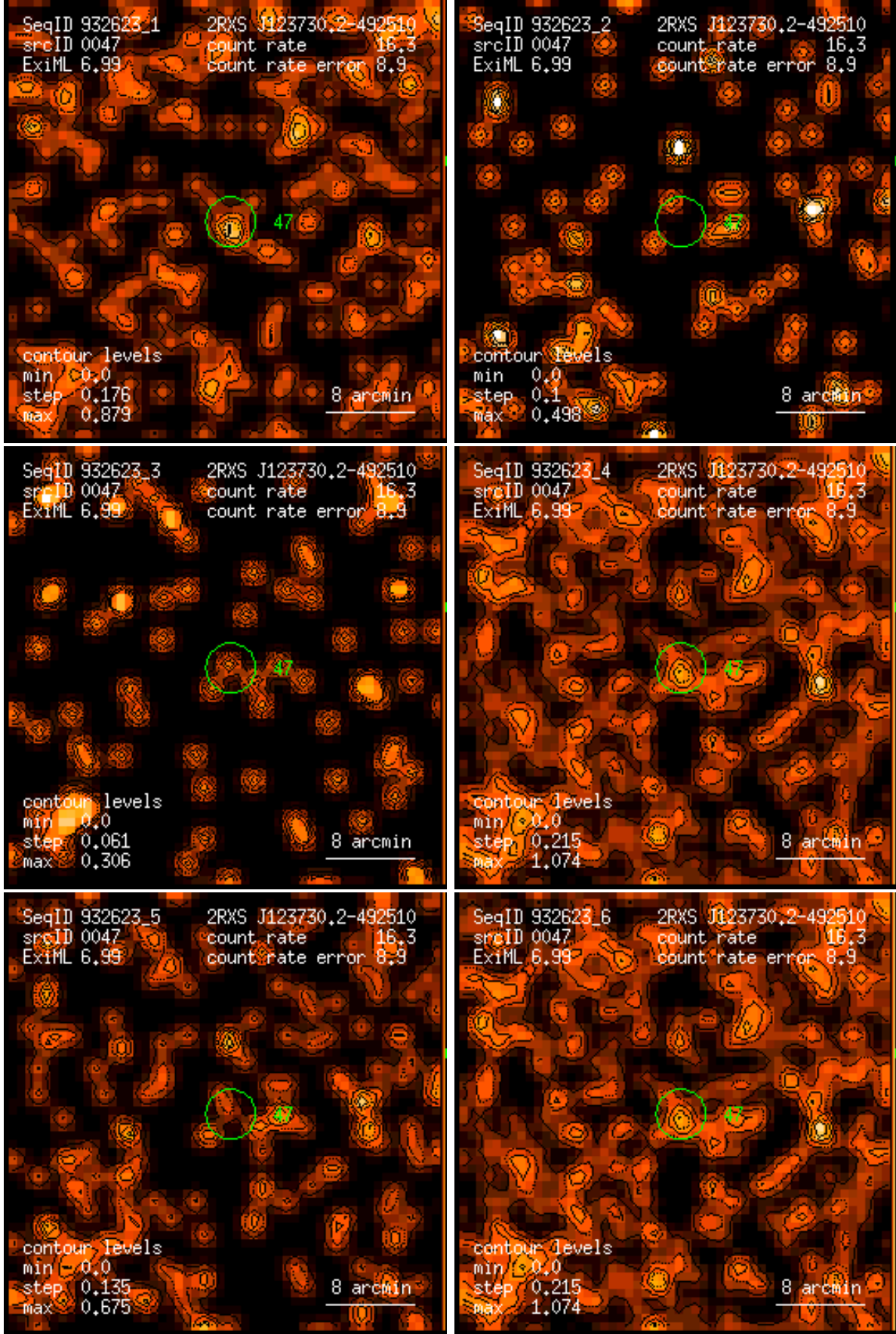
Figure 47: RASS 932623: detection 0047: band rate images, Gaussian filter: (1) PSPC channels 11 – 41, (2) 52 – 90, (3) 91 – 201, (4) 11 – 235, (5) 52 – 201, (6) 11 – 201. Broad band rates in counts/ks. Band rate contour levels in counts/ks/arcmin 2 .
