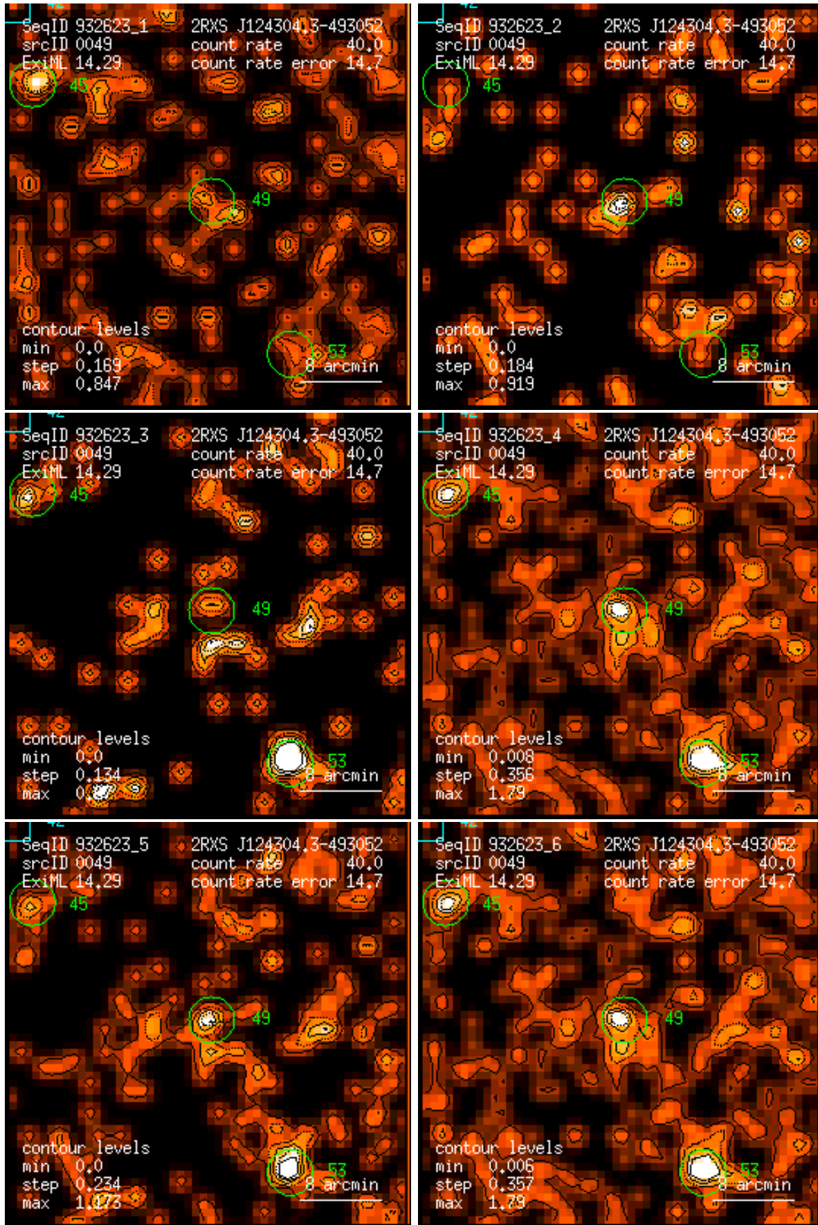
Figure 49: RASS 932623: detection 0049: band rate images, Gaussian filter: (1) PSPC channels 11 – 41, (2) 52 – 90, (3) 91 – 201, (4) 11 – 235, (5) 52 – 201, (6) 11 – 201. Broad band rates in counts/ks. Band rate contour levels in counts/ks/arcmin 2 .
