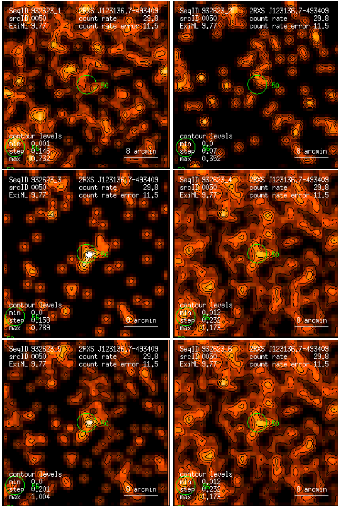
Figure 50: RASS 932623: detection 0050: band rate images, Gaussian filter: (1) PSPC channels 11 – 41, (2) 52 – 90, (3) 91 – 201, (4) 11 – 235, (5) 52 – 201, (6) 11 – 201. Broad band rates in counts/ks. Band rate contour levels in counts/ks/arcmin 2 .
