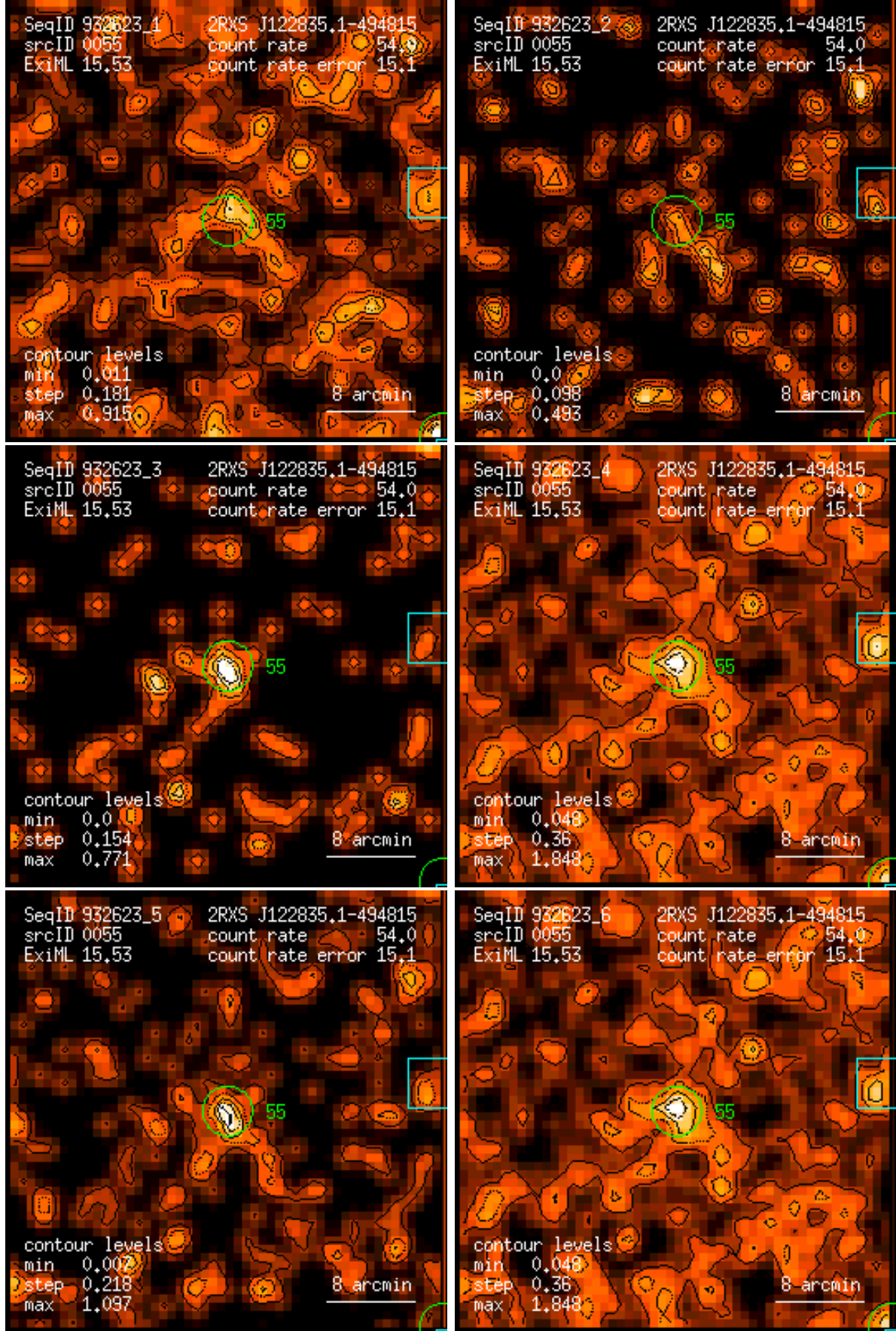
Figure 55: RASS 932623: detection 0055: band rate images, Gaussian filter: (1) PSPC channels 11 – 41, (2) 52 – 90, (3) 91 – 201, (4) 11 – 235, (5) 52 – 201, (6) 11 – 201. Broad band rates in counts/ks. Band rate contour levels in counts/ks/arcmin 2 .
