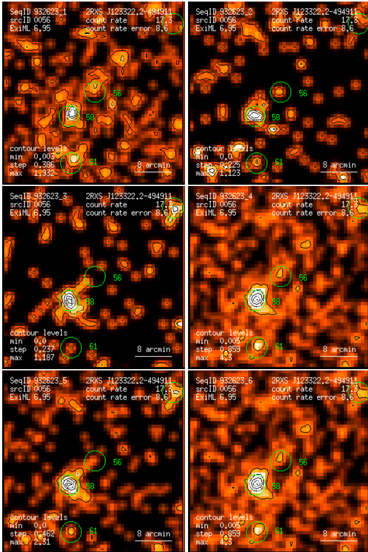
Figure 56: RASS 932623: detection 0056: band rate images, Gaussian filter: (1) PSPC channels 11 – 41, (2) 52 – 90, (3) 91 – 201, (4) 11 – 235, (5) 52 – 201, (6) 11 – 201. Broad band rates in counts/ks. Band rate contour levels in counts/ks/arcmin 2 .
