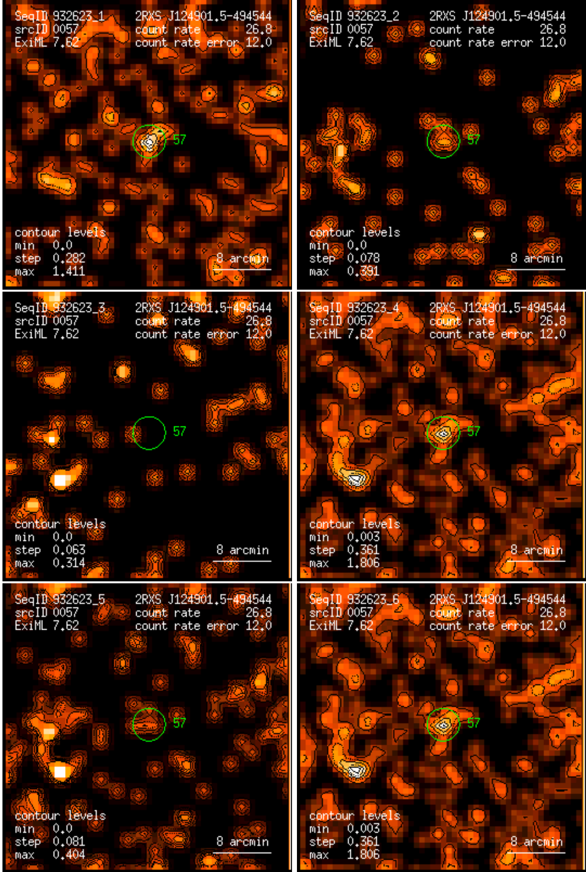
Figure 57: RASS 932623: detection 0057: band rate images, Gaussian filter: (1) PSPC channels 11 – 41, (2) 52 – 90, (3) 91 – 201, (4) 11 – 235, (5) 52 – 201, (6) 11 – 201. Broad band rates in counts/ks. Band rate contour levels in counts/ks/arcmin 2 .
