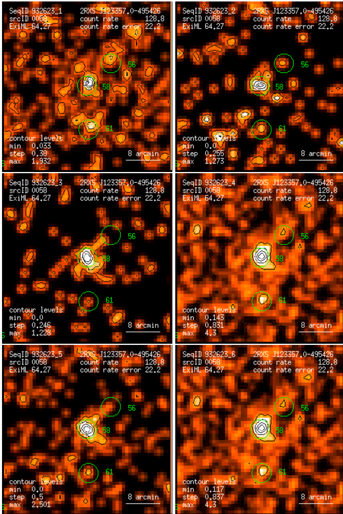
Figure 58: RASS 932623: detection 0058: band rate images, Gaussian filter: (1) PSPC channels 11 – 41, (2) 52 – 90, (3) 91 – 201, (4) 11 – 235, (5) 52 – 201, (6) 11 – 201. Broad band rates in counts/ks. Band rate contour levels in counts/ks/arcmin 2 .
