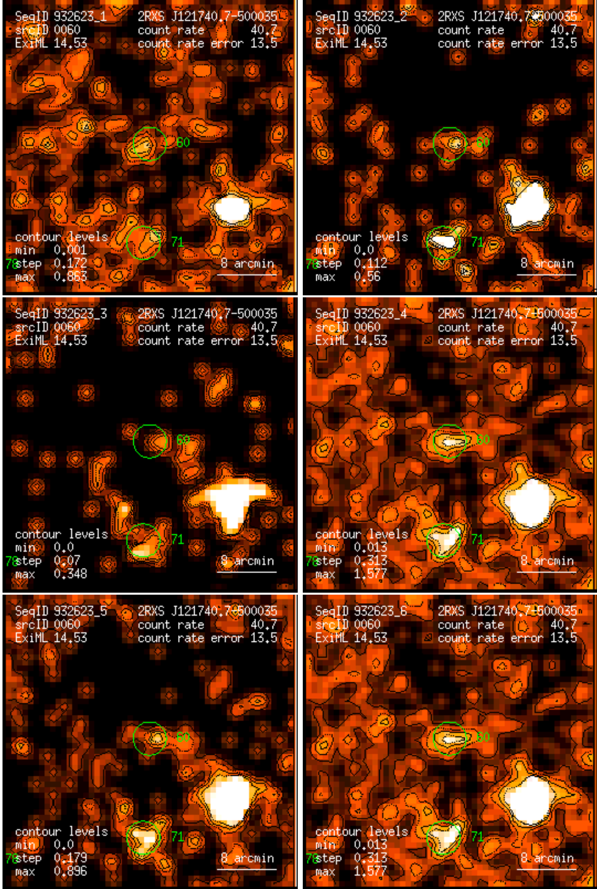
Figure 60: RASS 932623: detection 0060: band rate images, Gaussian filter: (1) PSPC channels 11 – 41, (2) 52 – 90, (3) 91 – 201, (4) 11 – 235, (5) 52 – 201, (6) 11 – 201. Broad band rates in counts/ks. Band rate contour levels in counts/ks/arcmin 2 .
