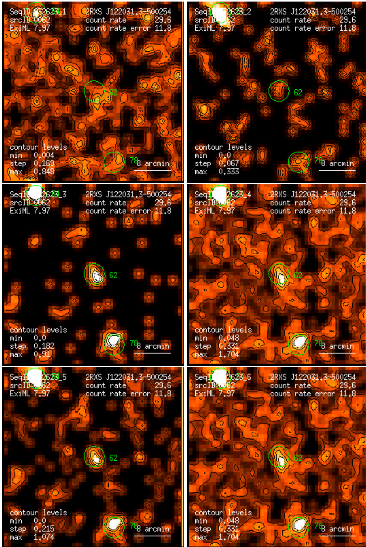
Figure 62: RASS 932623: detection 0062: band rate images, Gaussian filter: (1) PSPC channels 11 – 41, (2) 52 – 90, (3) 91 – 201, (4) 11 – 235, (5) 52 – 201, (6) 11 – 201. Broad band rates in counts/ks. Band rate contour levels in counts/ks/arcmin 2 .
