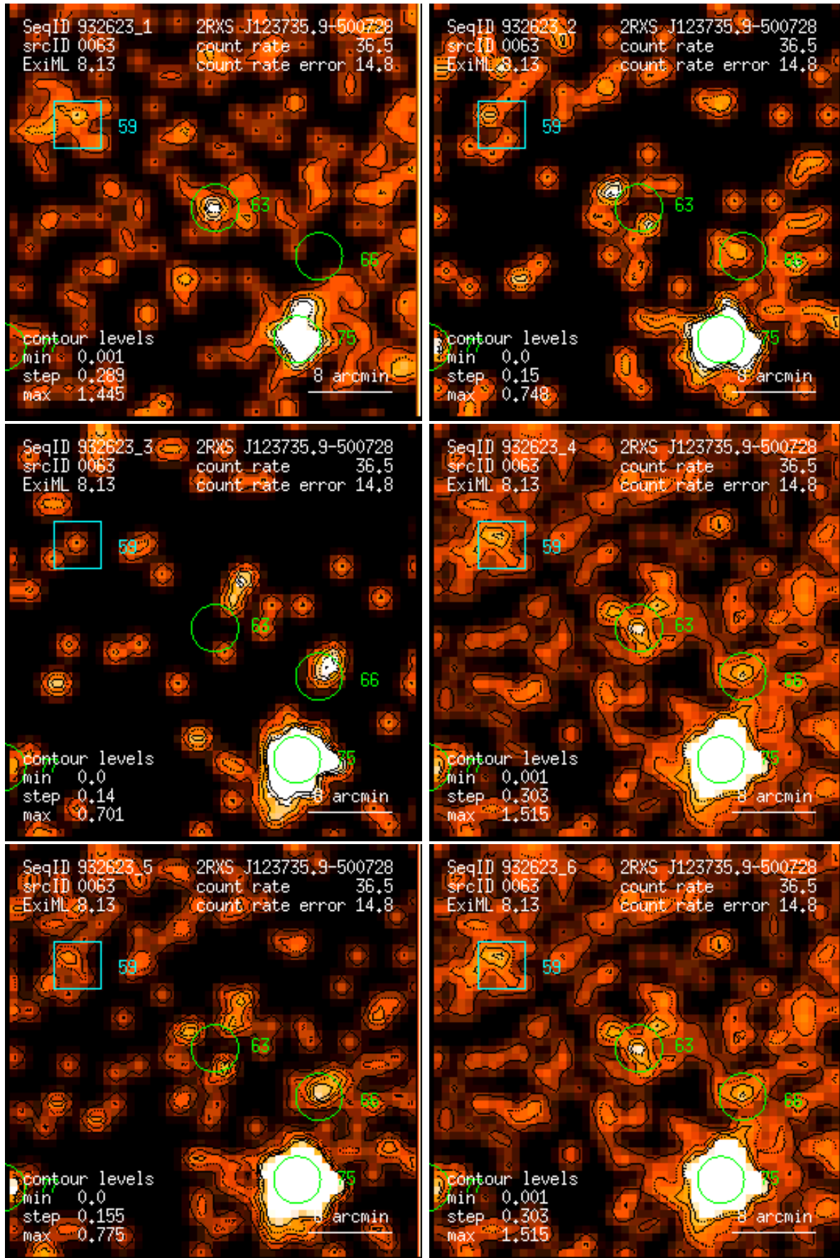
Figure 63: RASS 932623: detection 0063: band rate images, Gaussian filter: (1) PSPC channels 11 – 41, (2) 52 – 90, (3) 91 – 201, (4) 11 – 235, (5) 52 – 201, (6) 11 – 201. Broad band rates in counts/ks. Band rate contour levels in counts/ks/arcmin 2 .
