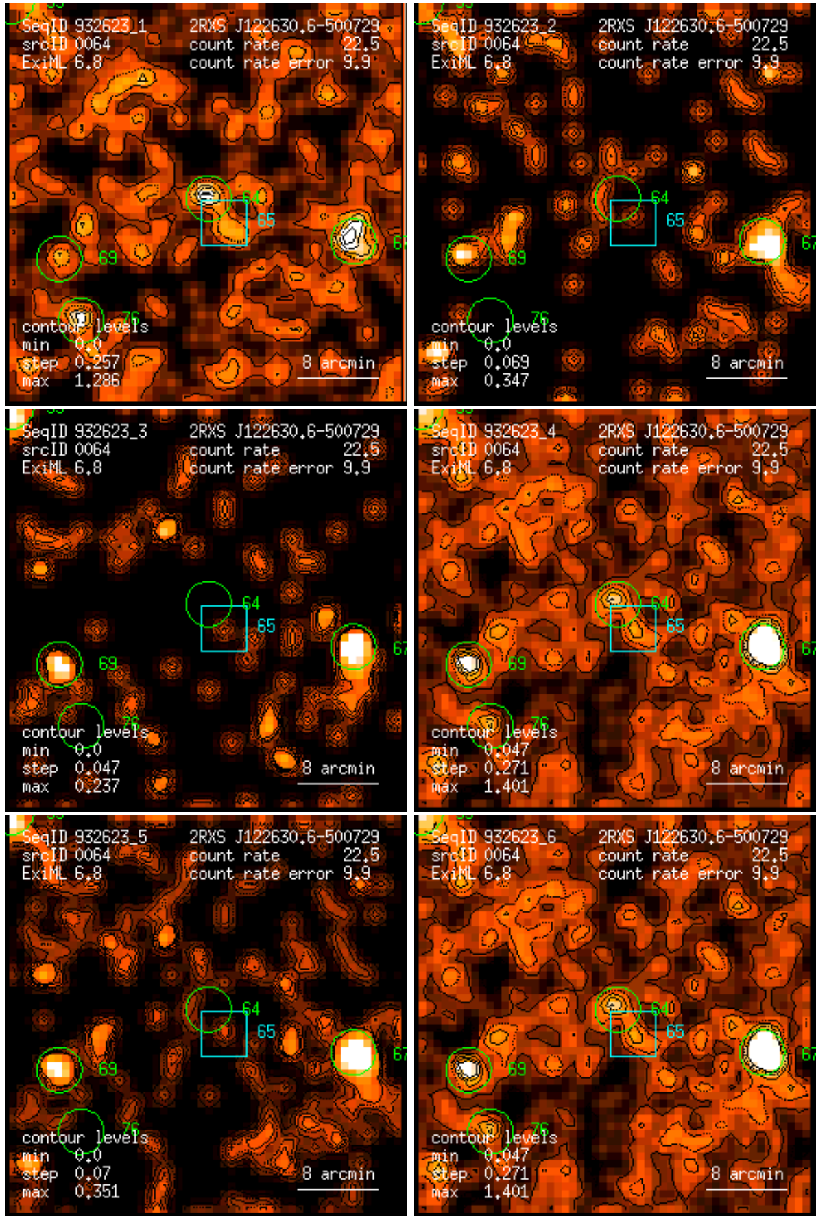
Figure 64: RASS 932623: detection 0064: band rate images, Gaussian filter: (1) PSPC channels 11 – 41, (2) 52 – 90, (3) 91 – 201, (4) 11 – 235, (5) 52 – 201, (6) 11 – 201. Broad band rates in counts/ks. Band rate contour levels in counts/ks/arcmin 2 .
