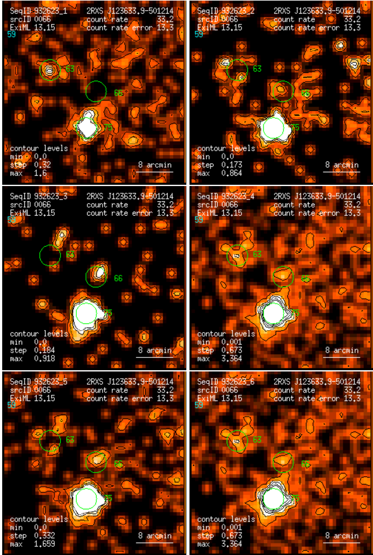
Figure 66: RASS 932623: detection 0066: band rate images, Gaussian filter: (1) PSPC channels 11 – 41, (2) 52 – 90, (3) 91 – 201, (4) 11 – 235, (5) 52 – 201, (6) 11 – 201. Broad band rates in counts/ks. Band rate contour levels in counts/ks/arcmin 2 .
