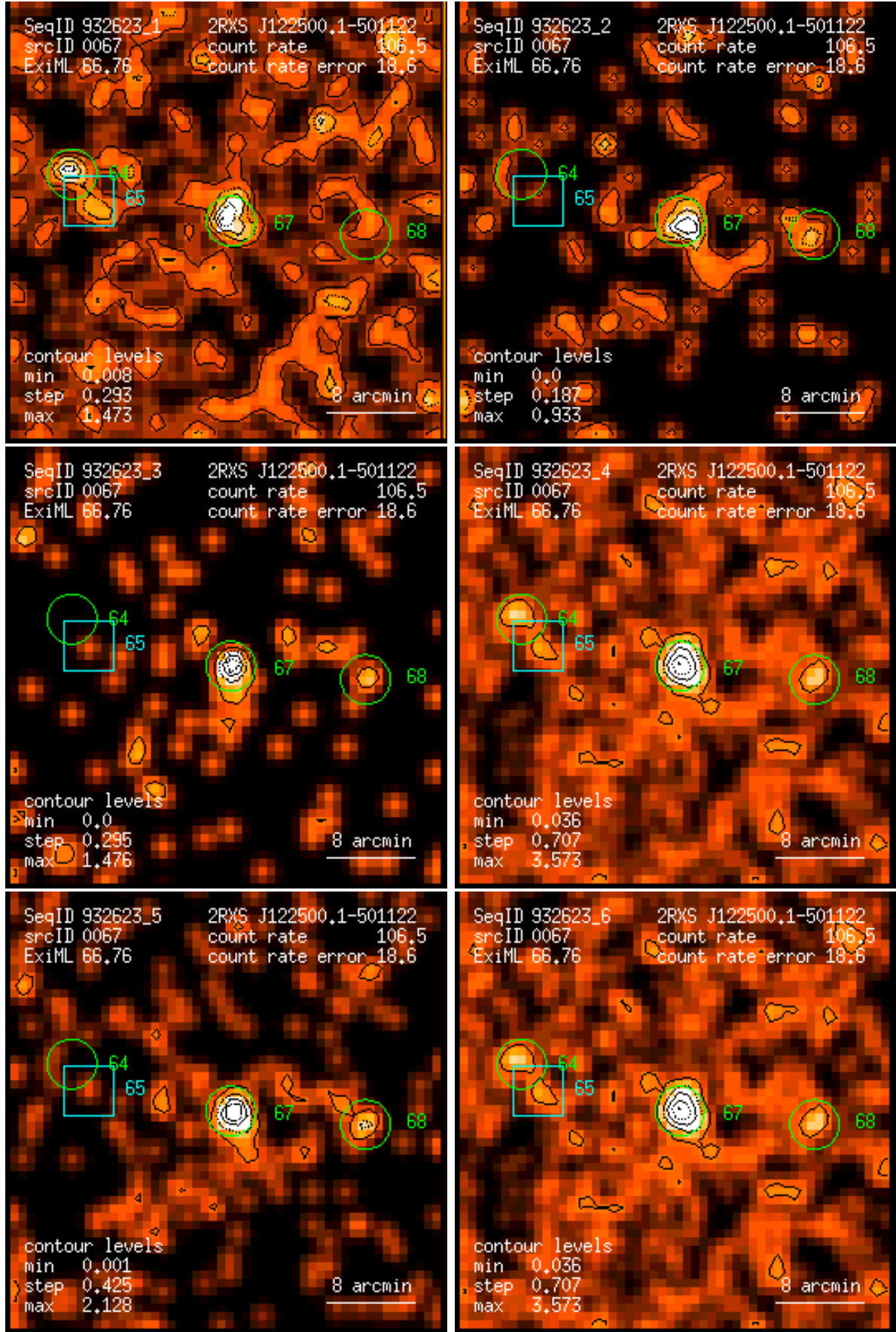
Figure 67: RASS 932623: detection 0067: band rate images, Gaussian filter: (1) PSPC channels 11 – 41, (2) 52 – 90, (3) 91 – 201, (4) 11 – 235, (5) 52 – 201, (6) 11 – 201. Broad band rates in counts/ks. Band rate contour levels in counts/ks/arcmin 2 .
