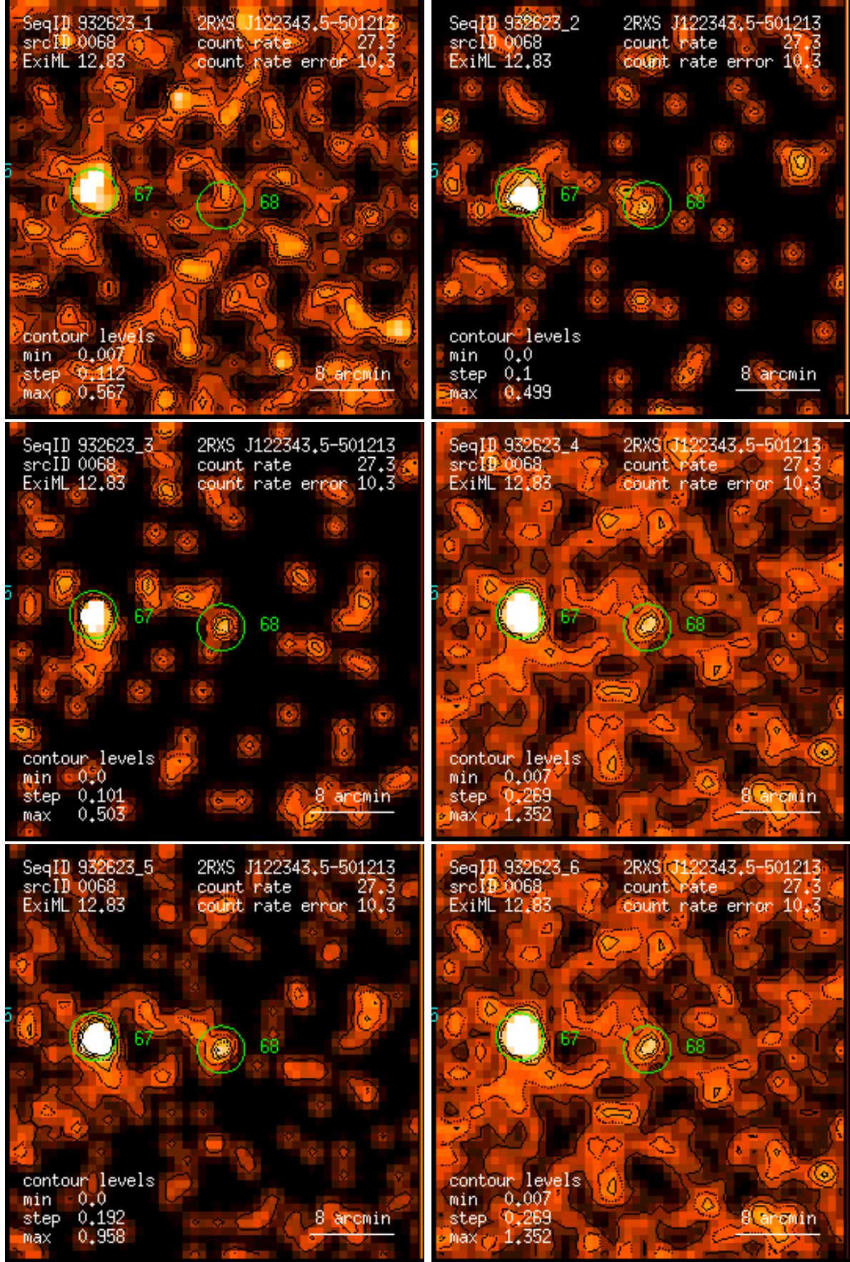
Figure 68: RASS 932623: detection 0068: band rate images, Gaussian filter: (1) PSPC channels 11 – 41, (2) 52 – 90, (3) 91 – 201, (4) 11 – 235, (5) 52 – 201, (6) 11 – 201. Broad band rates in counts/ks. Band rate contour levels in counts/ks/arcmin 2 .
