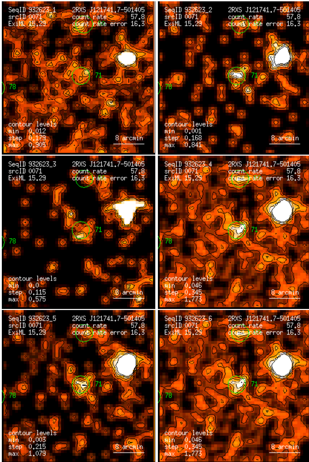
Figure 71: RASS 932623: detection 0071: band rate images, Gaussian filter: (1) PSPC channels 11 – 41, (2) 52 – 90, (3) 91 – 201, (4) 11 – 235, (5) 52 – 201, (6) 11 – 201. Broad band rates in counts/ks. Band rate contour levels in counts/ks/arcmin 2 .
