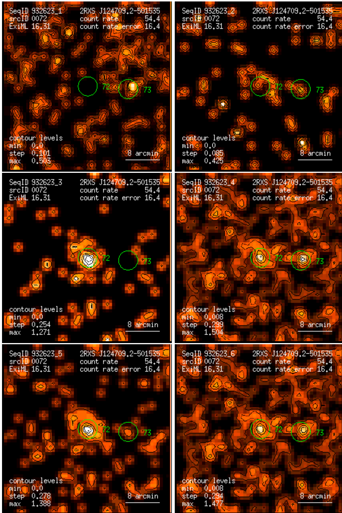
Figure 72: RASS 932623: detection 0072: band rate images, Gaussian filter: (1) PSPC channels 11 – 41, (2) 52 – 90, (3) 91 – 201, (4) 11 – 235, (5) 52 – 201, (6) 11 – 201. Broad band rates in counts/ks. Band rate contour levels in counts/ks/arcmin 2 .
