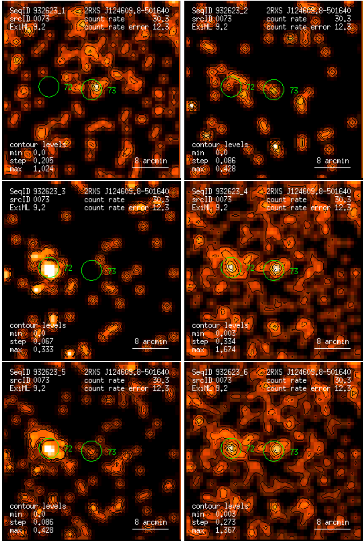
Figure 73: RASS 932623: detection 0073: band rate images, Gaussian filter: (1) PSPC channels 11 – 41, (2) 52 – 90, (3) 91 – 201, (4) 11 – 235, (5) 52 – 201, (6) 11 – 201. Broad band rates in counts/ks. Band rate contour levels in counts/ks/arcmin 2 .
