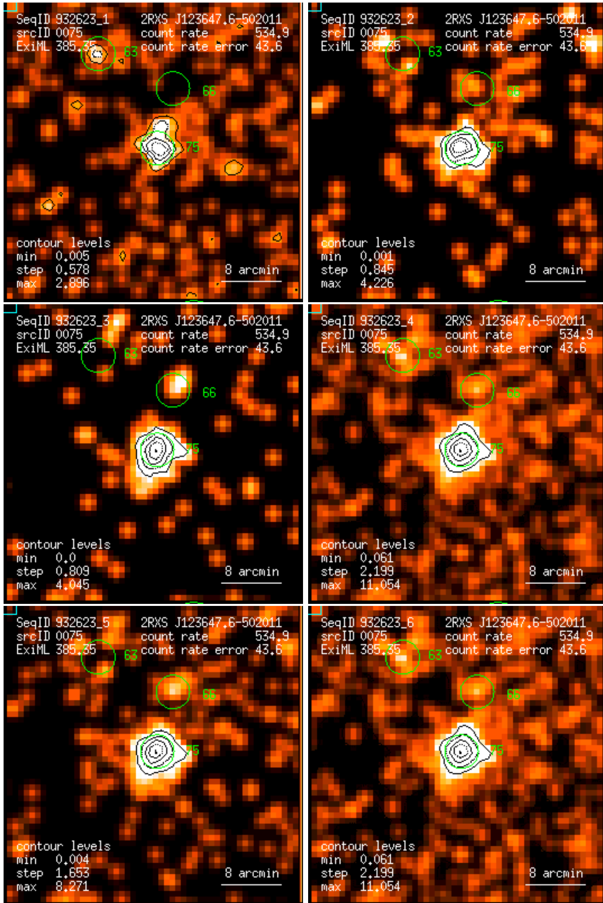
Figure 75: RASS 932623: detection 0075: band rate images, Gaussian filter: (1) PSPC channels 11 – 41, (2) 52 – 90, (3) 91 – 201, (4) 11 – 235, (5) 52 – 201, (6) 11 – 201. Broad band rates in counts/ks. Band rate contour levels in counts/ks/arcmin 2 .
