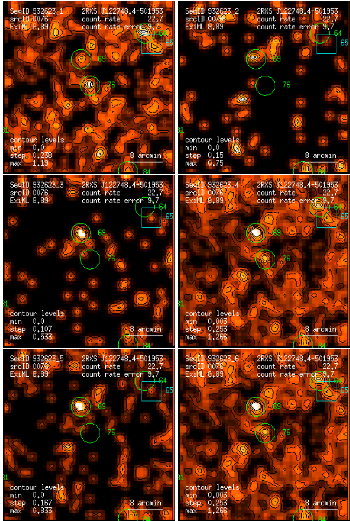
Figure 76: RASS 932623: detection 0076: band rate images, Gaussian filter: (1) PSPC channels 11 – 41, (2) 52 – 90, (3) 91 – 201, (4) 11 – 235, (5) 52 – 201, (6) 11 – 201. Broad band rates in counts/ks. Band rate contour levels in counts/ks/arcmin 2 .
