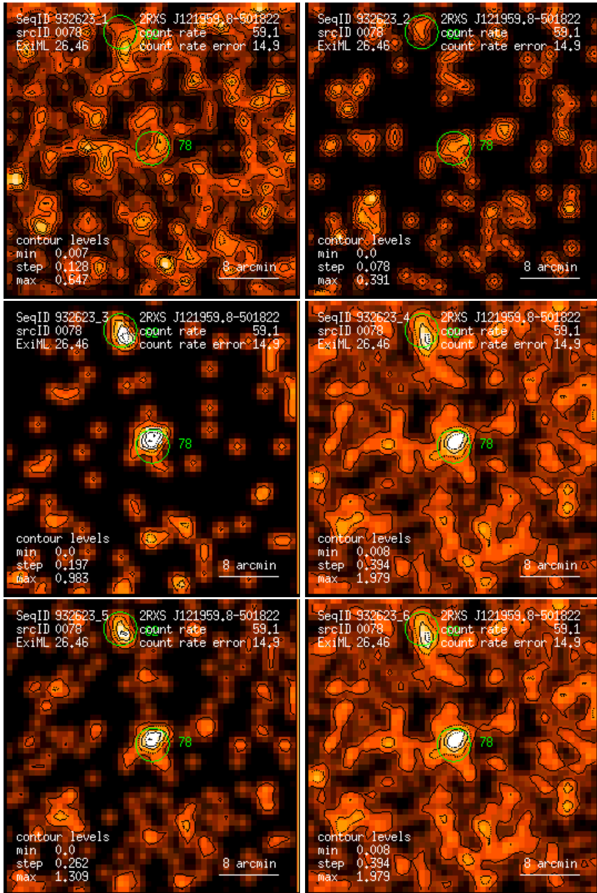
Figure 78: RASS 932623: detection 0078: band rate images, Gaussian filter: (1) PSPC channels 11 – 41, (2) 52 – 90, (3) 91 – 201, (4) 11 – 235, (5) 52 – 201, (6) 11 – 201. Broad band rates in counts/ks. Band rate contour levels in counts/ks/arcmin 2 .
