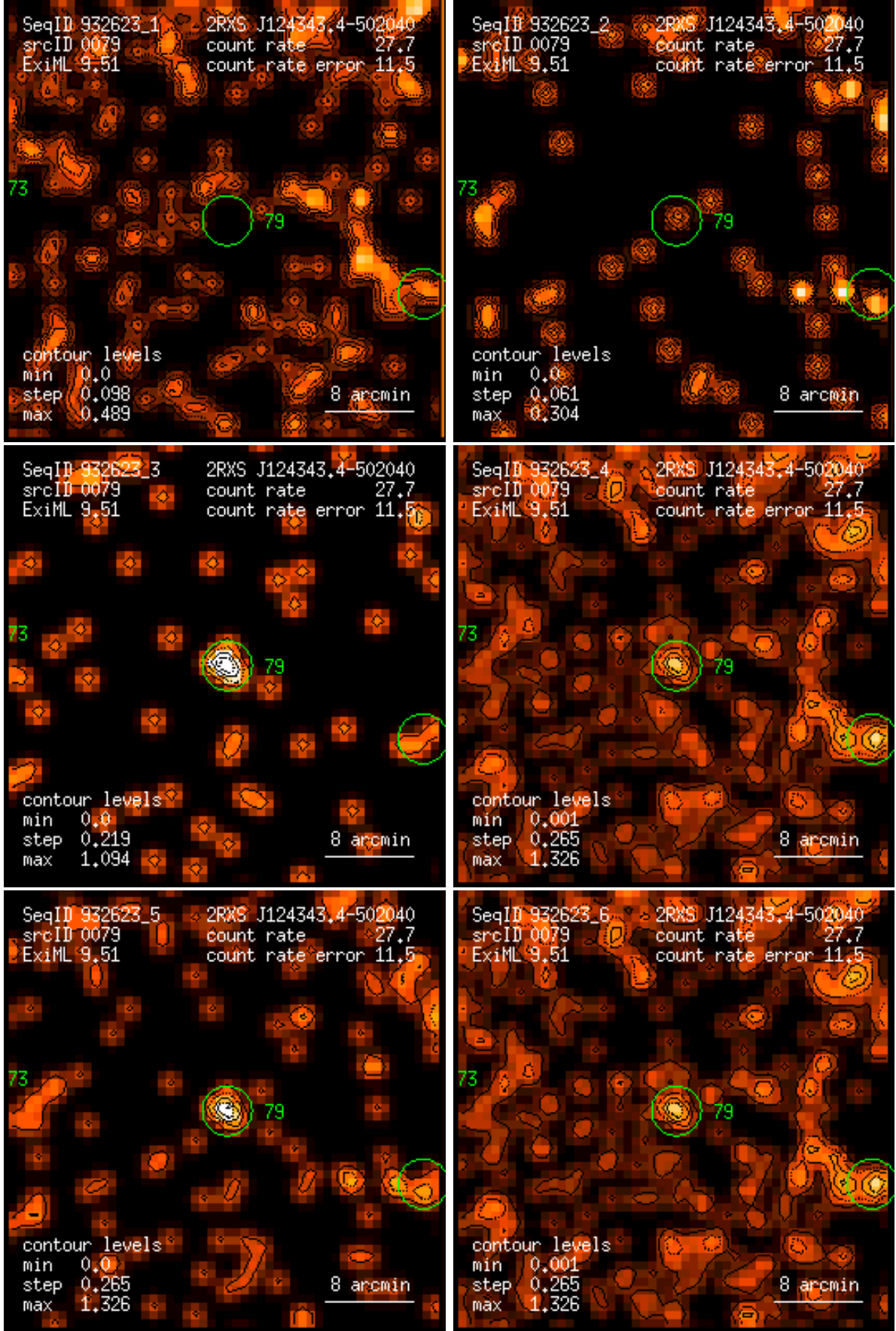
Figure 79: RASS 932623: detection 0079: band rate images, Gaussian filter: (1) PSPC channels 11 – 41, (2) 52 – 90, (3) 91 – 201, (4) 11 – 235, (5) 52 – 201, (6) 11 – 201. Broad band rates in counts/ks. Band rate contour levels in counts/ks/arcmin 2 .
